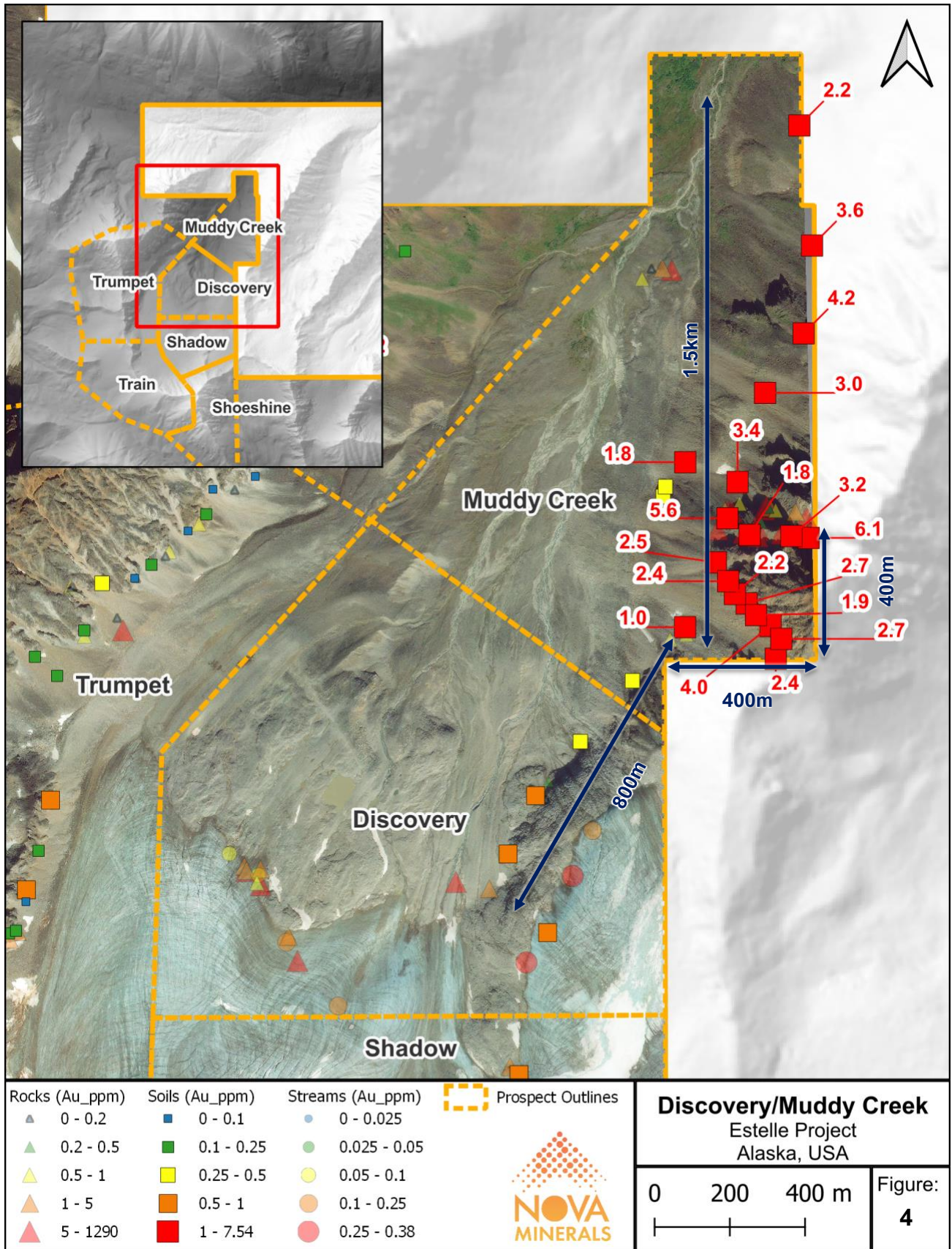
Figure 4. Discovery and Muddy Creek gold anomalies
