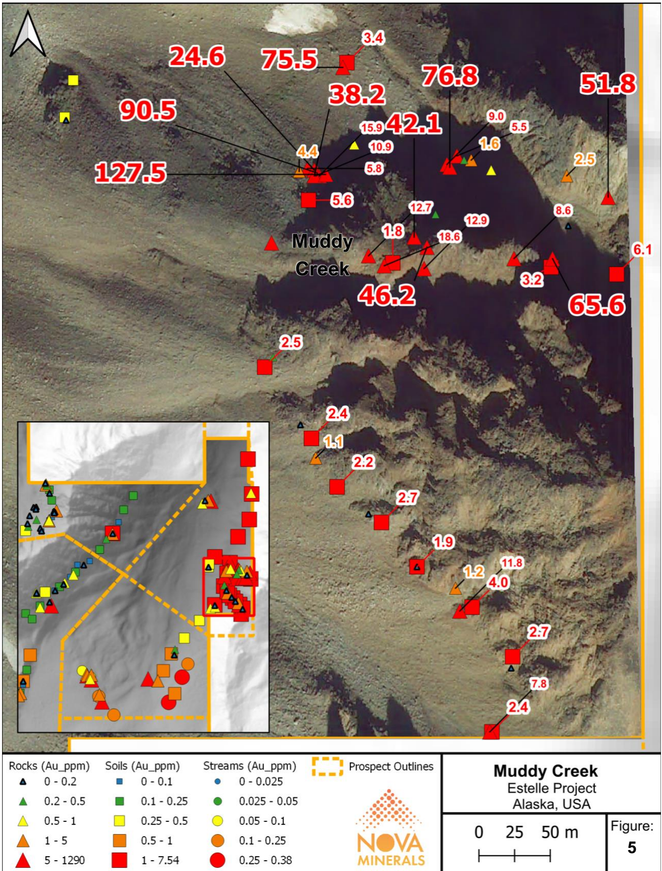
Figure 5. Muddy Creek core zone Au sample results plan view map
