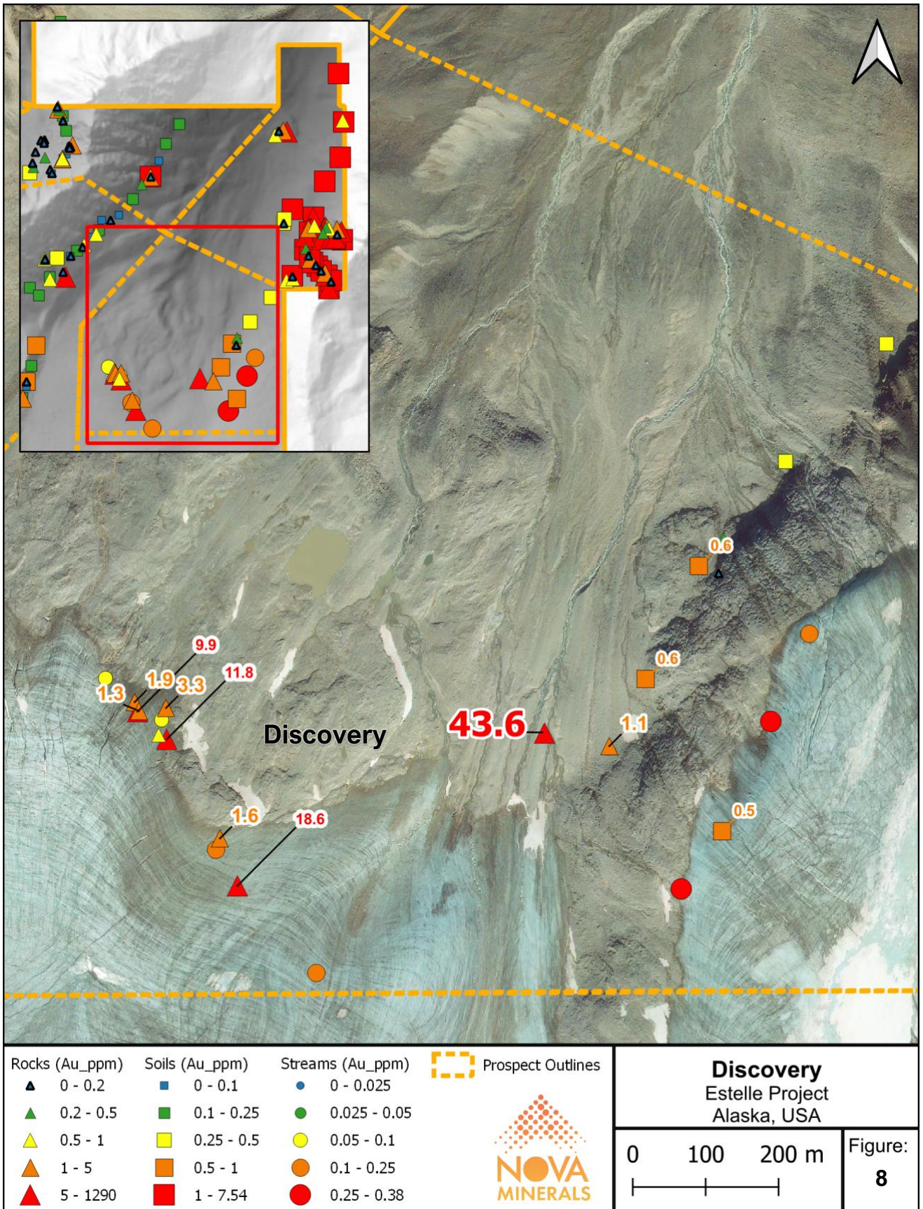
Figure 8. Discovery Au sample results plan view map
