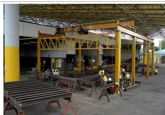
Fabrication area for Safe Live Process Plant
