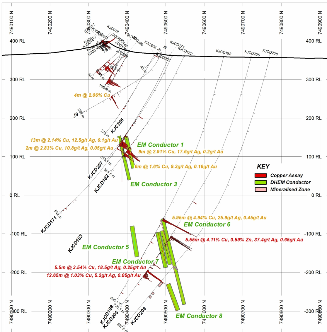
Figure 1 Rockface Cross Section 628360E Showing KJCD205, KJC206, KJCD207 & KJCD208
