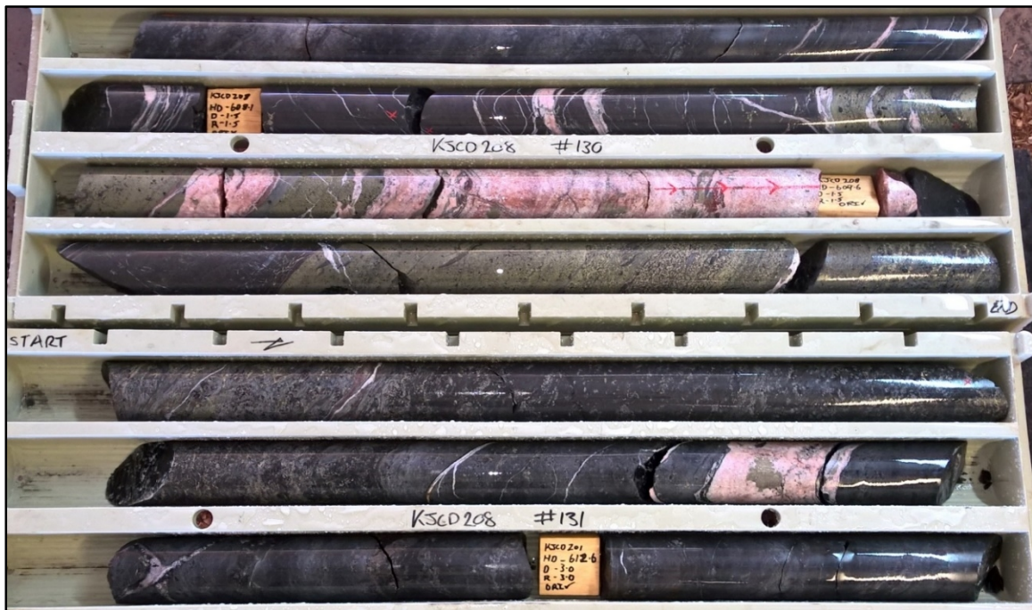
Photograph 3 - Mineralised diamond drill core from KJCD208 (circa 610m) showing interpreted Conductor 6 massive and disseminated sulphide mineralisation
