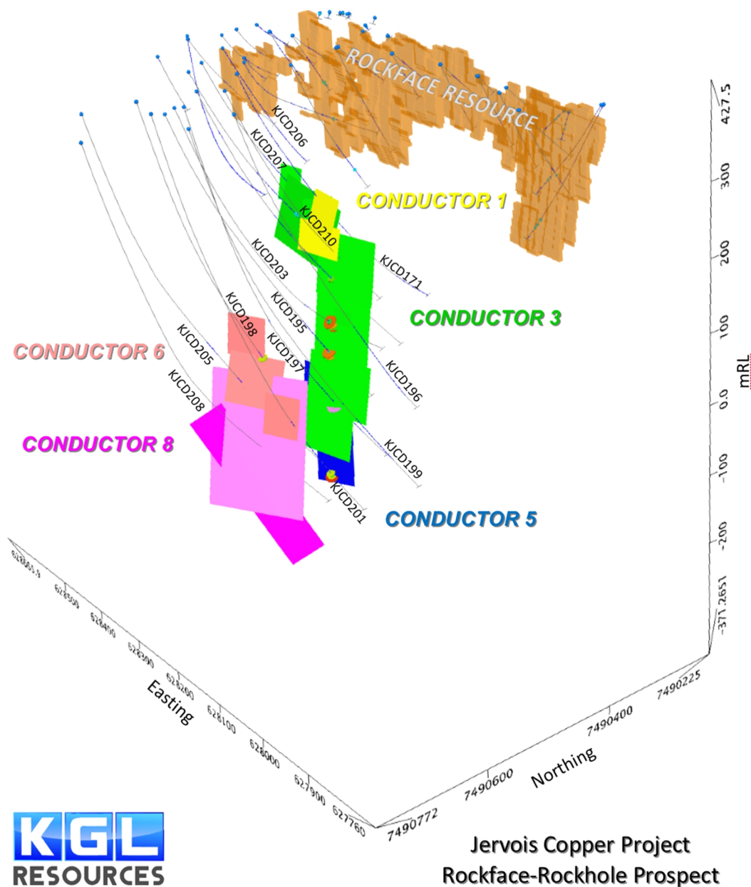
Figure 4 Rockface DHEM Conductors (looking SE)
