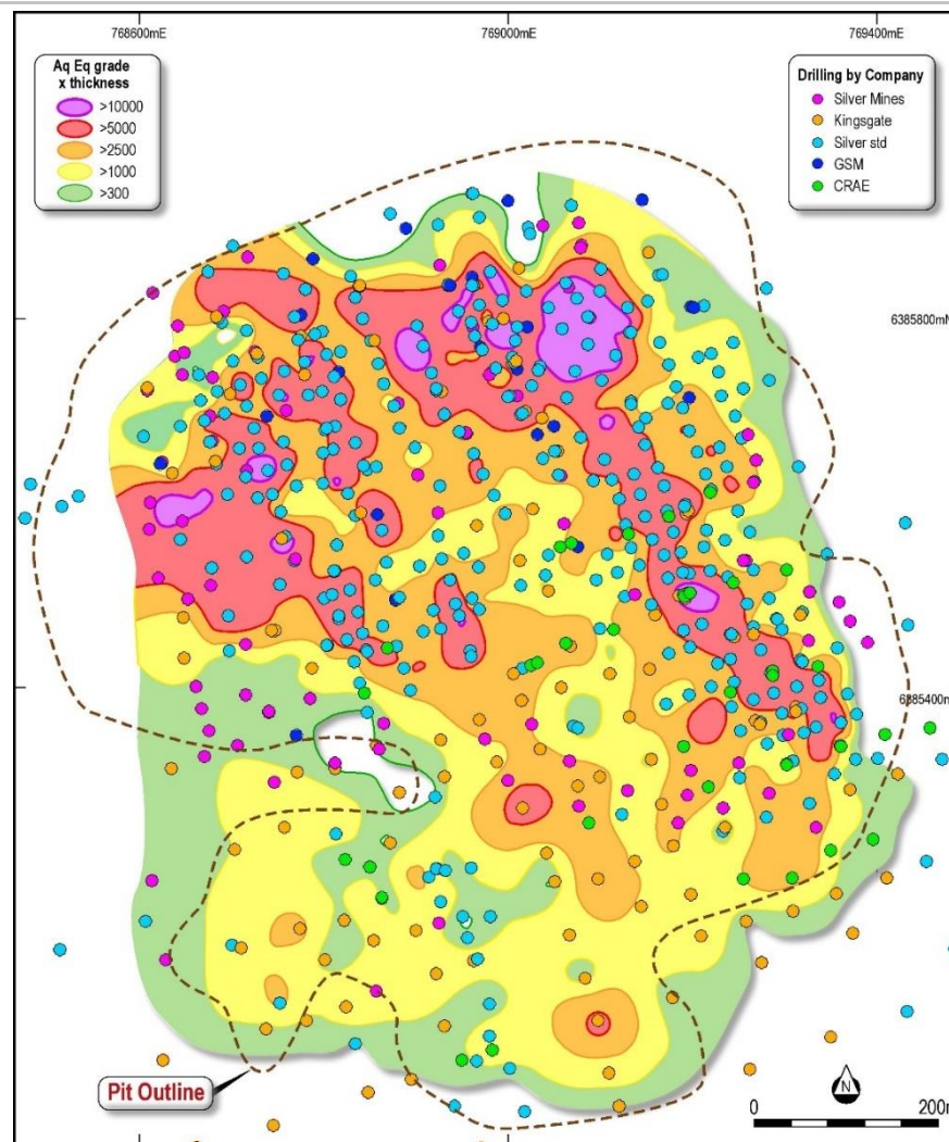
Grade thickness map based on previous resource.
