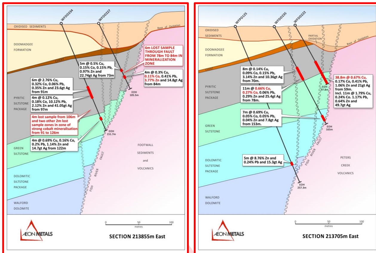
Figure 3: Sections for holes WFDD234 and WFDD235
