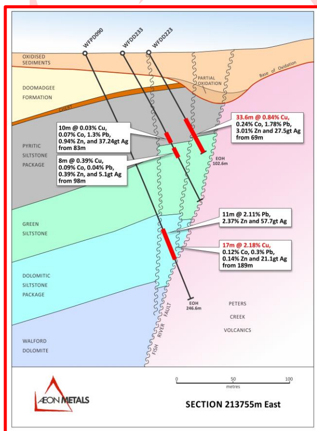
Figure 4: Section for Hole WFDD233
