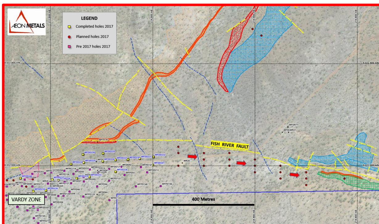
Figure 1: Walford drill plan showing currently completed diamond holes. Zone trending east of Vardy now being tested by RC drilling over at least 800m to locate Fish River fault and set up pre-collars for diamond drill holes.
