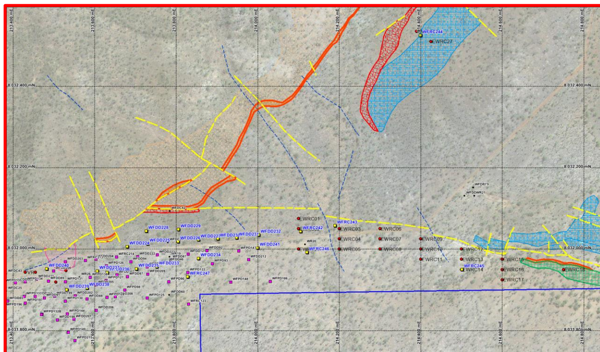
Figure 1: Walford drill plan showing currently completed diamond and RC holes completed to test eastward extension of the Fish River Fault.
