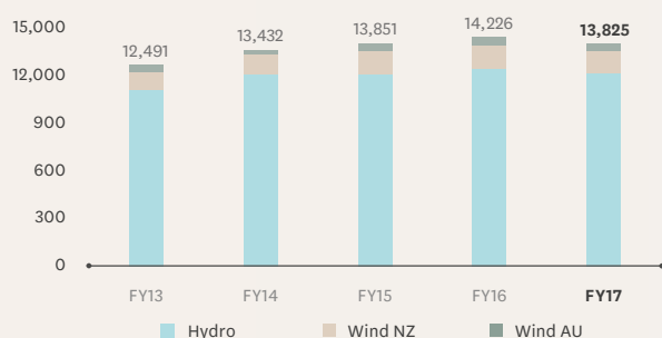
GENERATION (GWh 8 )
