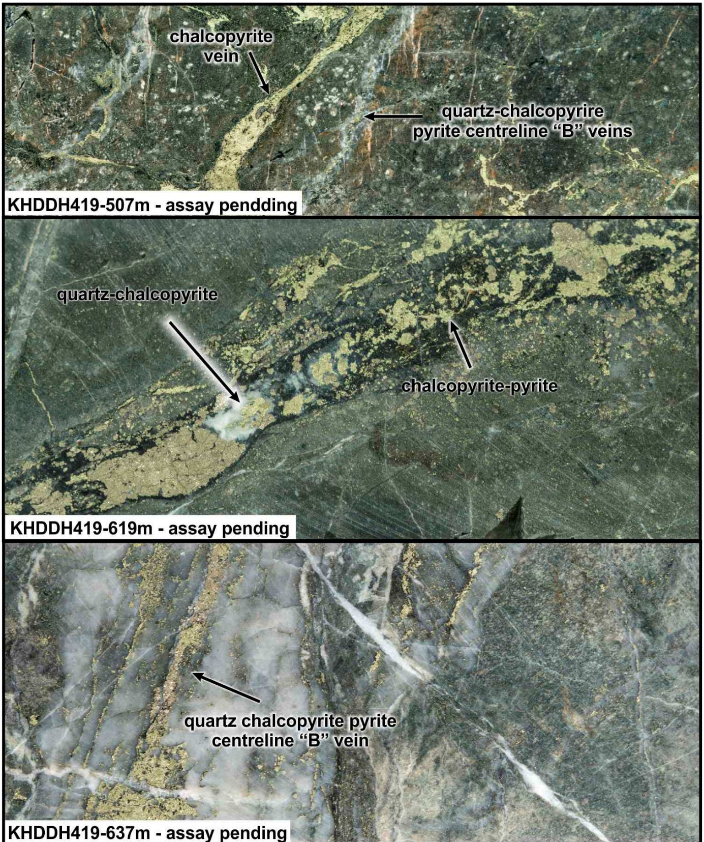
FIGURE 7: Mineralisation from drill hole KHDDH419. Halved HQ core, the height of each image is 6.35cm. Assays pending.
