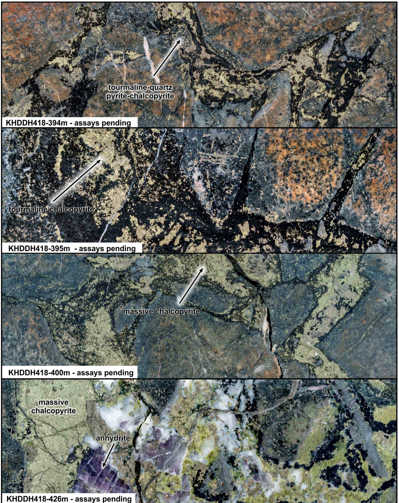
FIGURE 6: Mineralisation from drill hole KHDDH418. Halved HQ core, the height of each image is 6.35cm. Assays pending.
