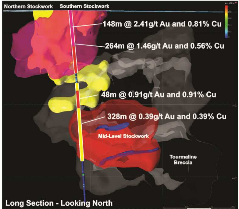
FIGURE 3: 3D geological model of Stockwork Hill showing the key geological features and the location of drill hole KHDDH415.
