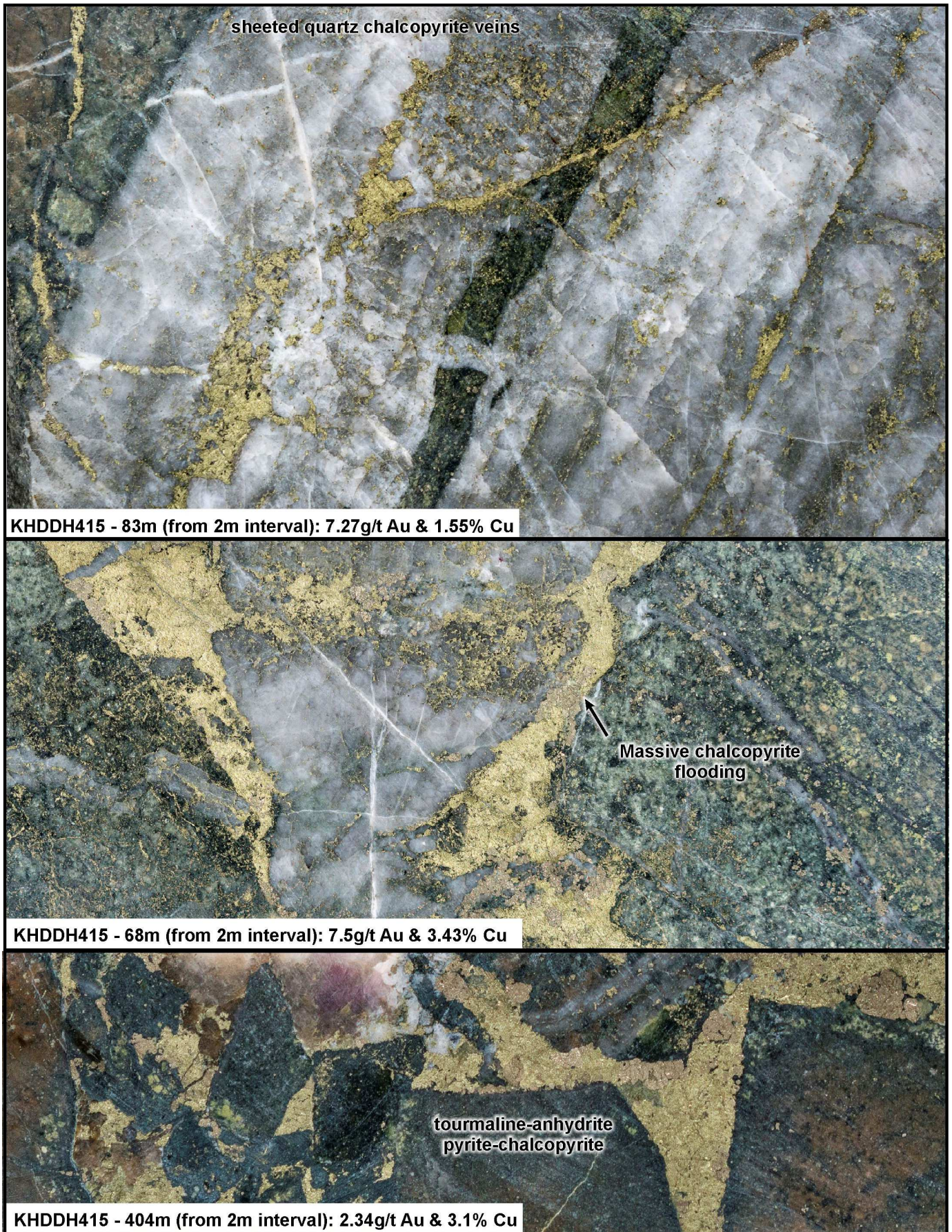
FIGURE 4: Mineralisation from drill hole KHDDH415. Halved HQ core, the height of each image is 6.35cm.
