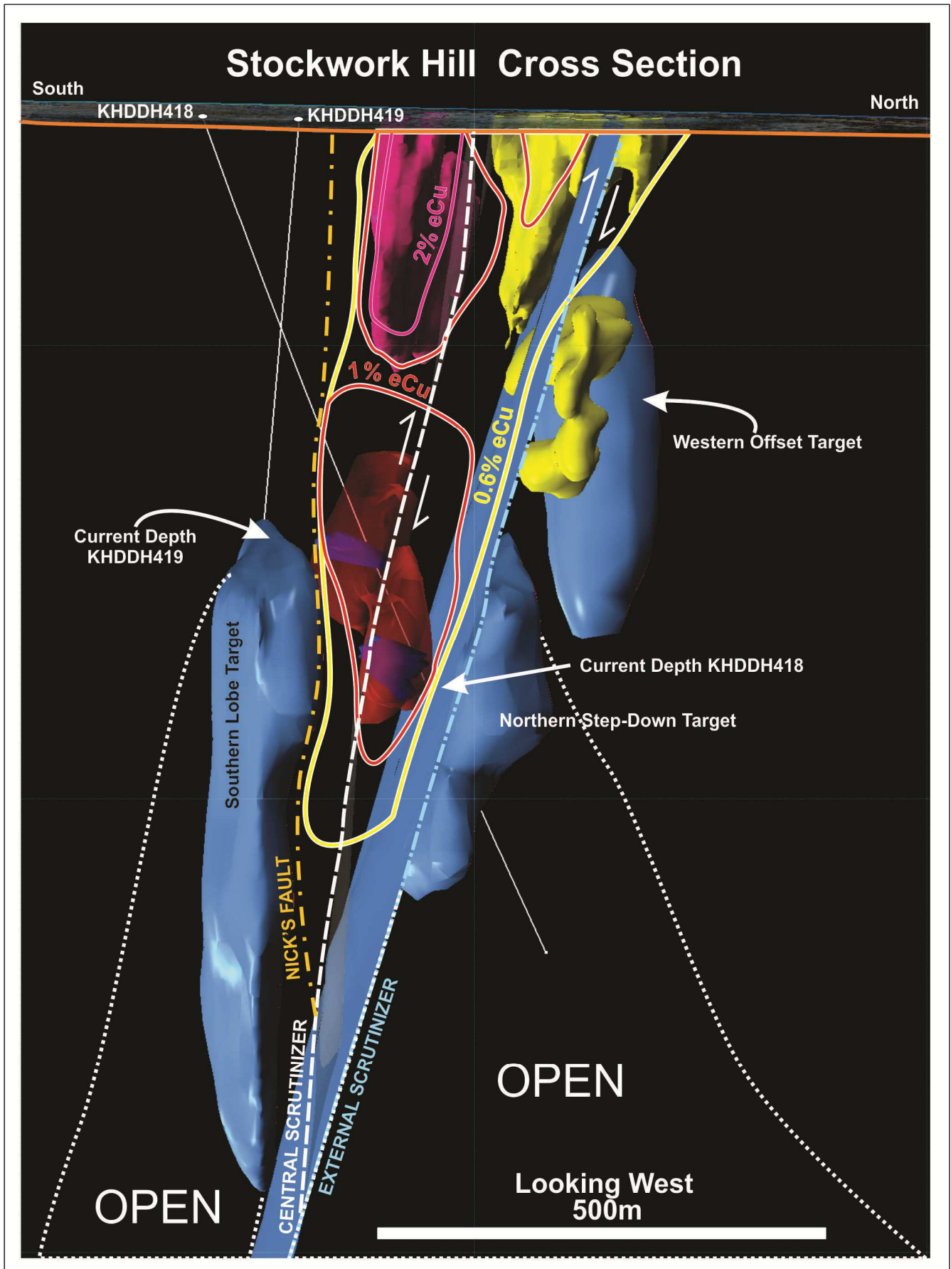
FIGURE 5: 3D geological model of the Stockwork Hill Deposit defining new high-grade targets.
