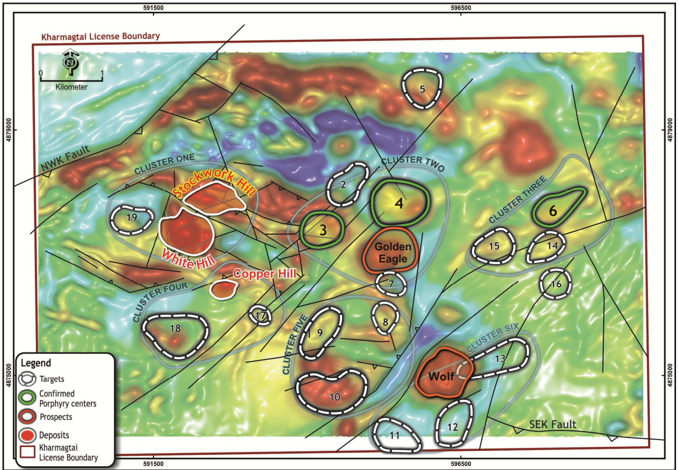
FIGURE 2: The Kharmagtai Mining Licence showing ground magnetic data and location of the Stockwork Hill Deposit.
