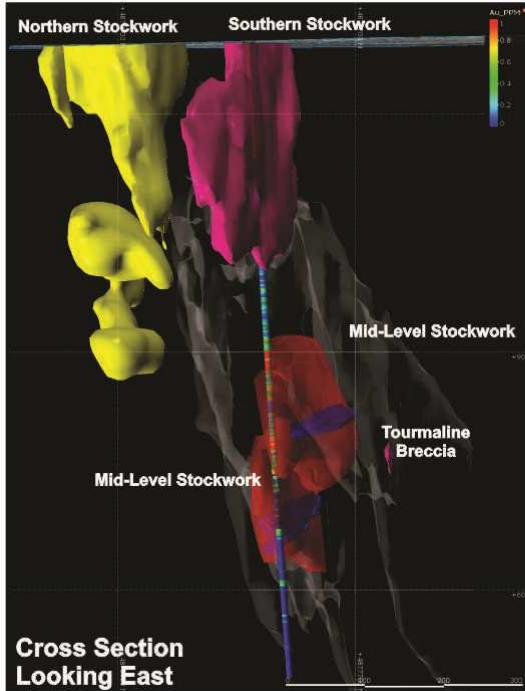
FIGURE 3: 3D geological model of Stockwork Hill showing the key geological features and the location of drill hole KHDDH415.
