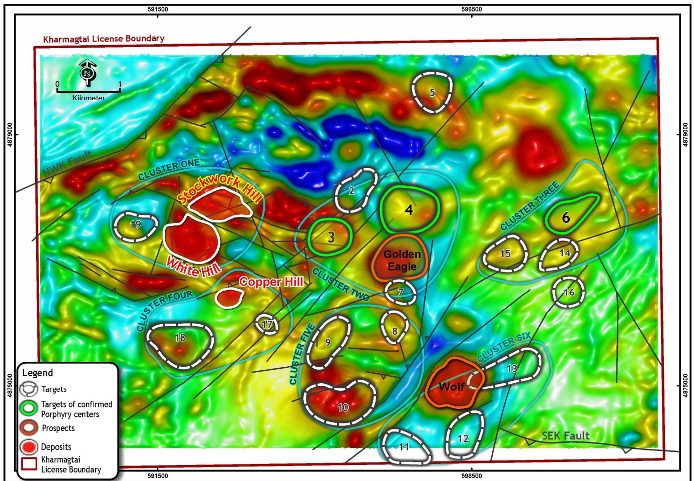
FIGURE 2: The Kharmagtai Mining Licence ground magnetic data and known porphyry deposits with newly confirmed porphyry systems.
