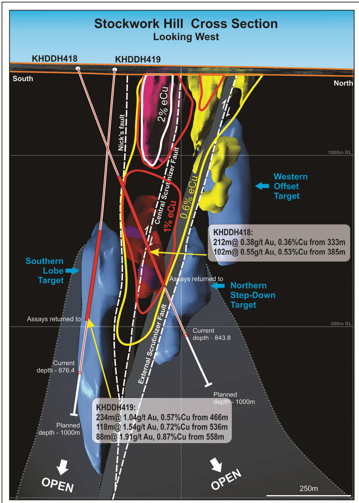
FIGURE 3: Cross section through the 3D geological model of the Stockwork Hill Deposit showing the location of the three new extensional targets (light blue).
