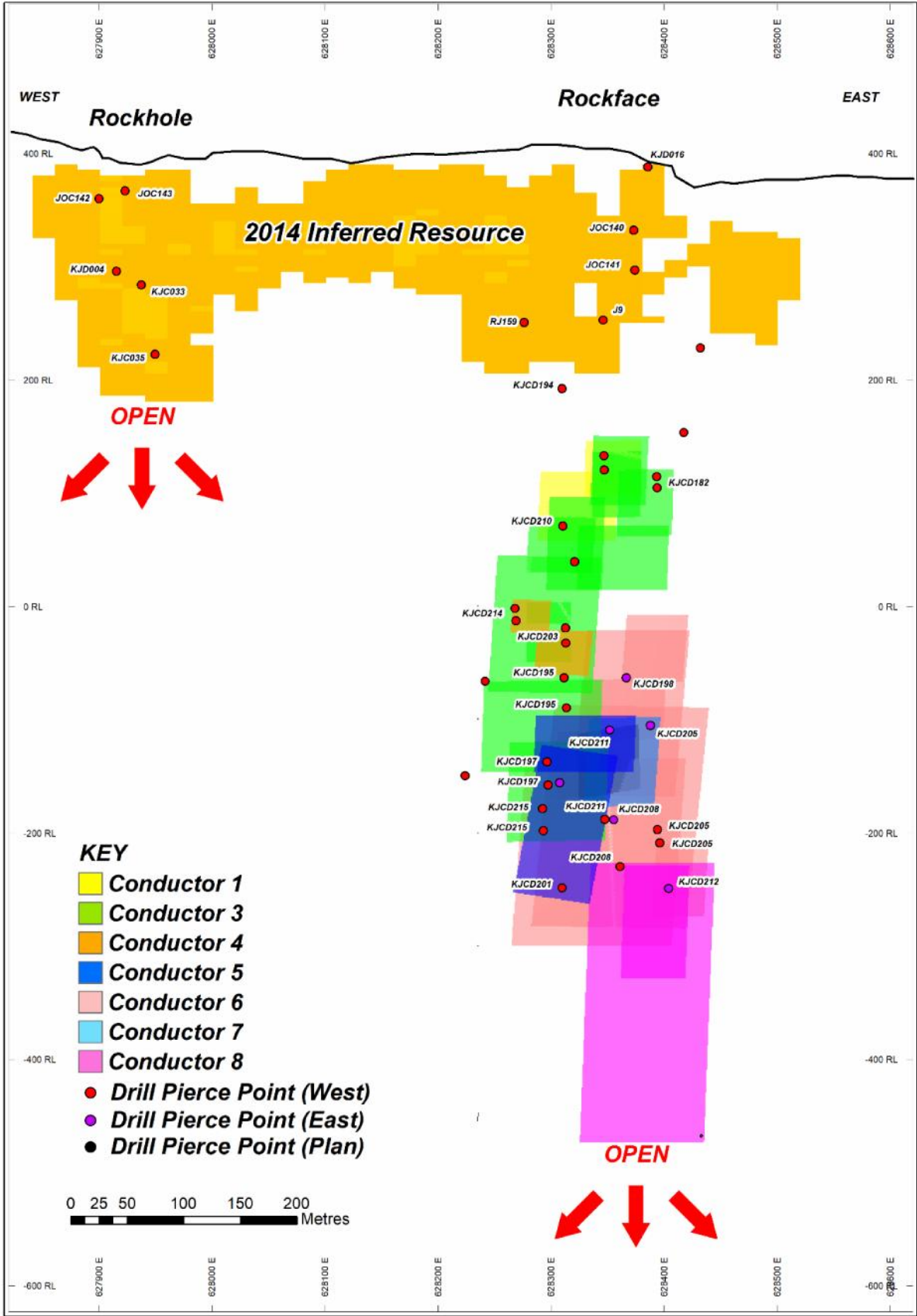
Figure 3 Rockface Long section
