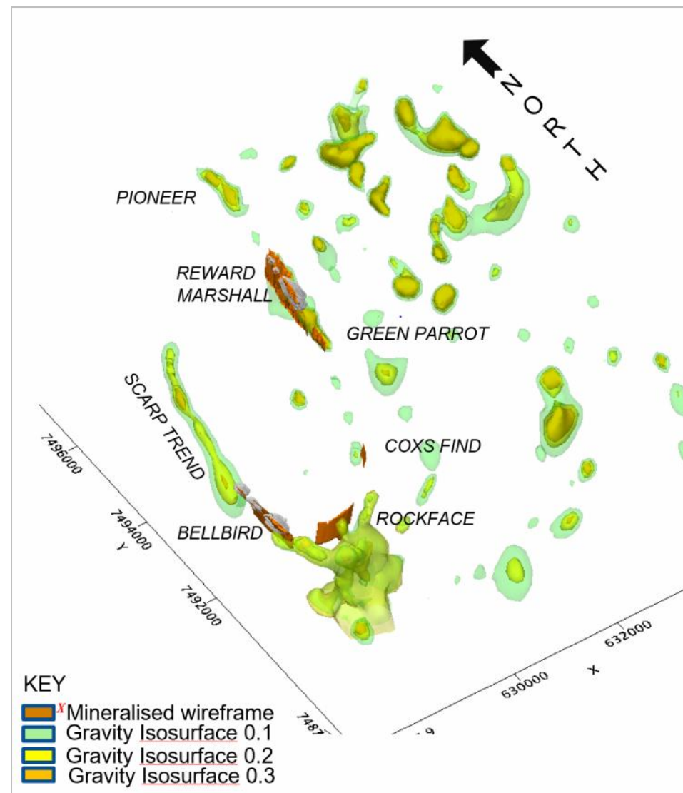
Figure 5 Gravity inversion isosurfaces for Jervois and Unca Creek
