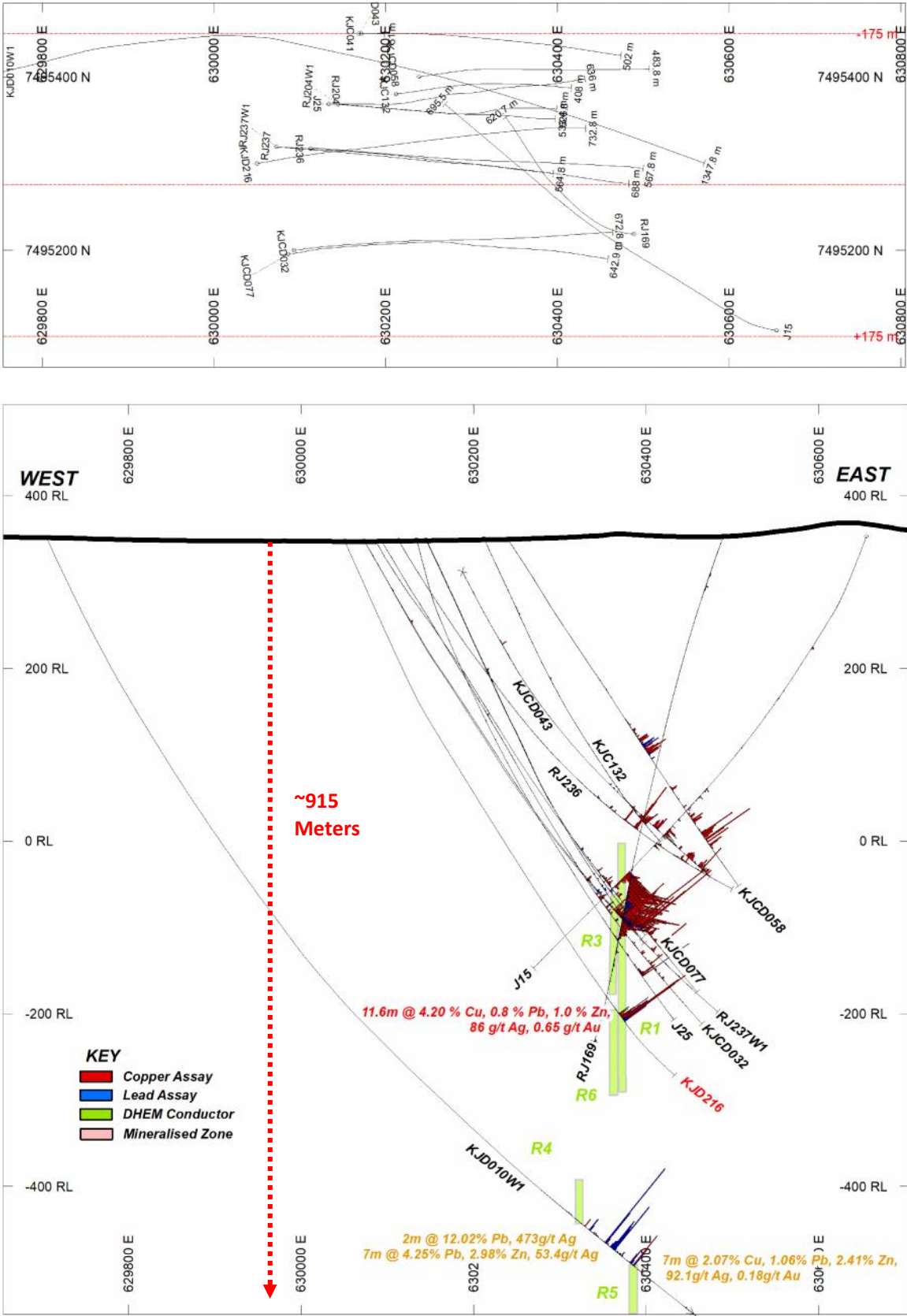
Figure 1. Reward Cross-Section 7495275N
