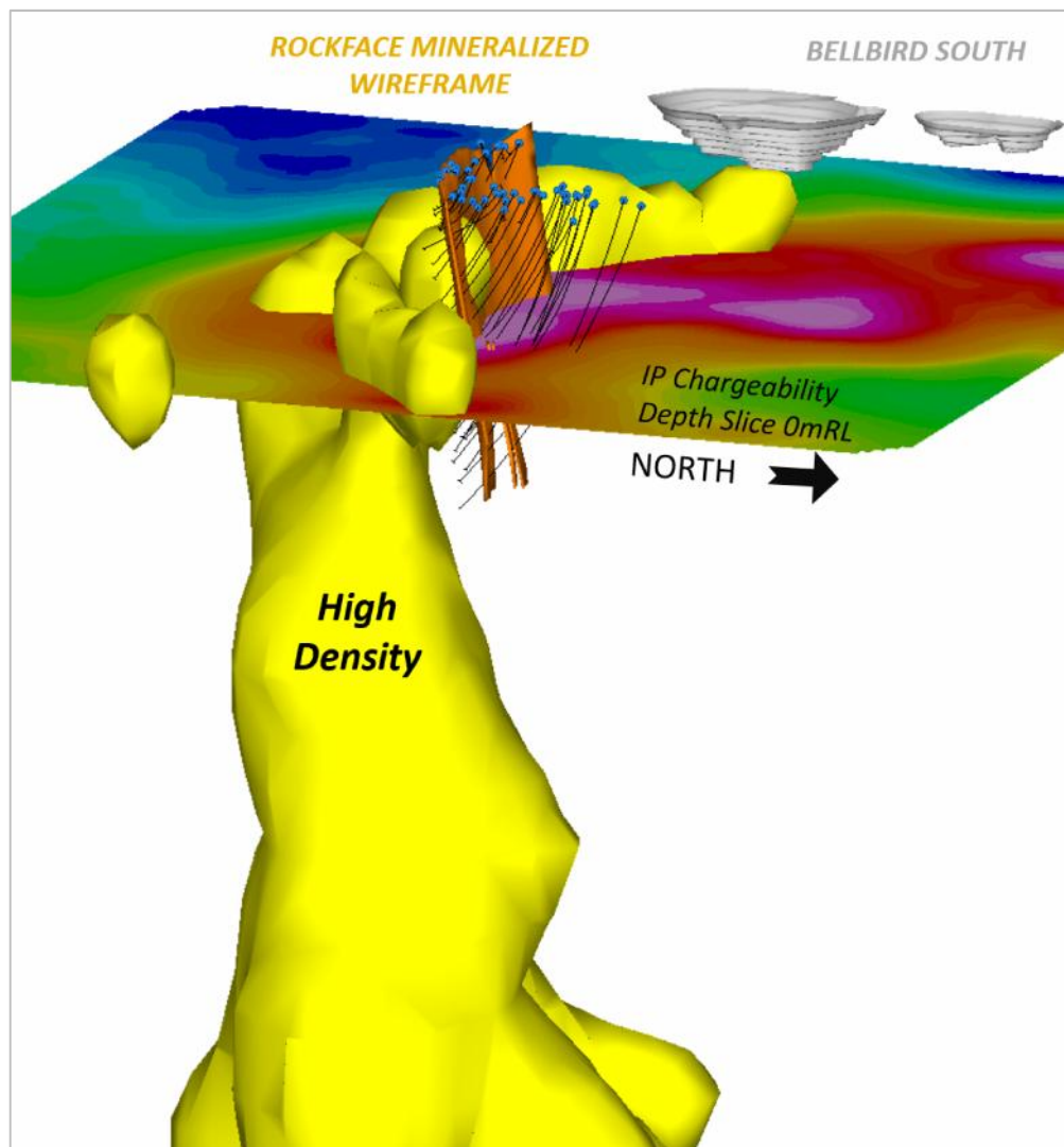
Gravity inversion – Bellbird and Rockface region
