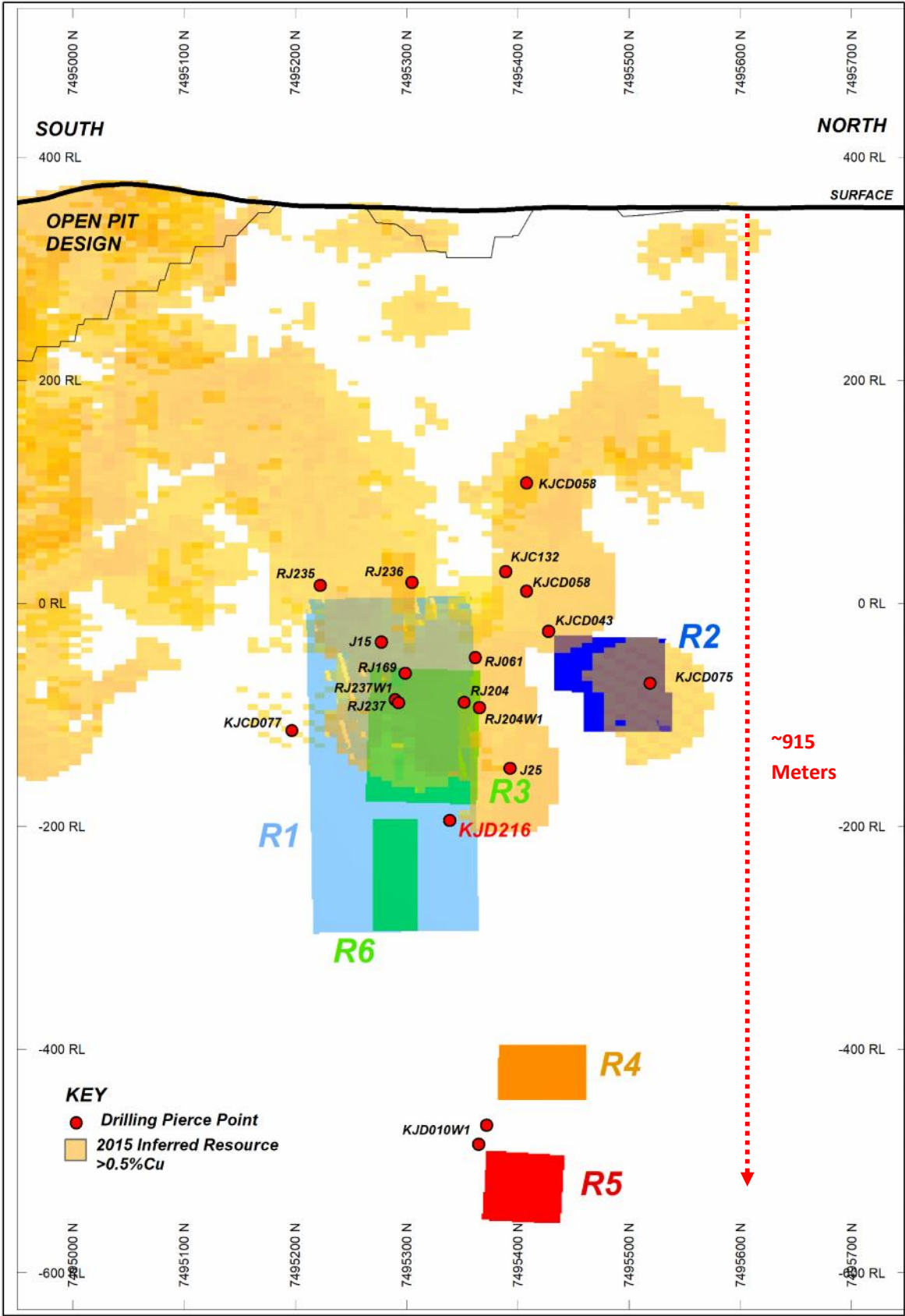
Figure 2 Reward Long section 630 380E highlighting the DHEM conductors
