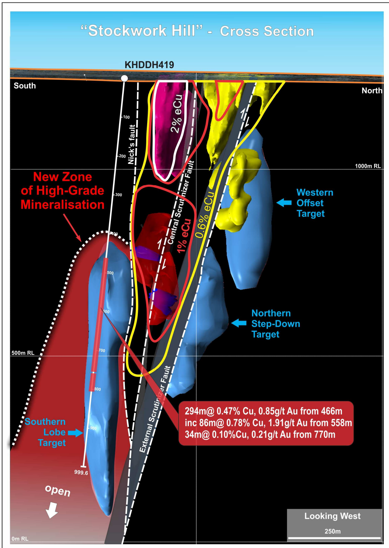
FIGURE 5: Cross section of Stockwork Hill showing the Southern Lobe Target and drill hole KHDDH419.
