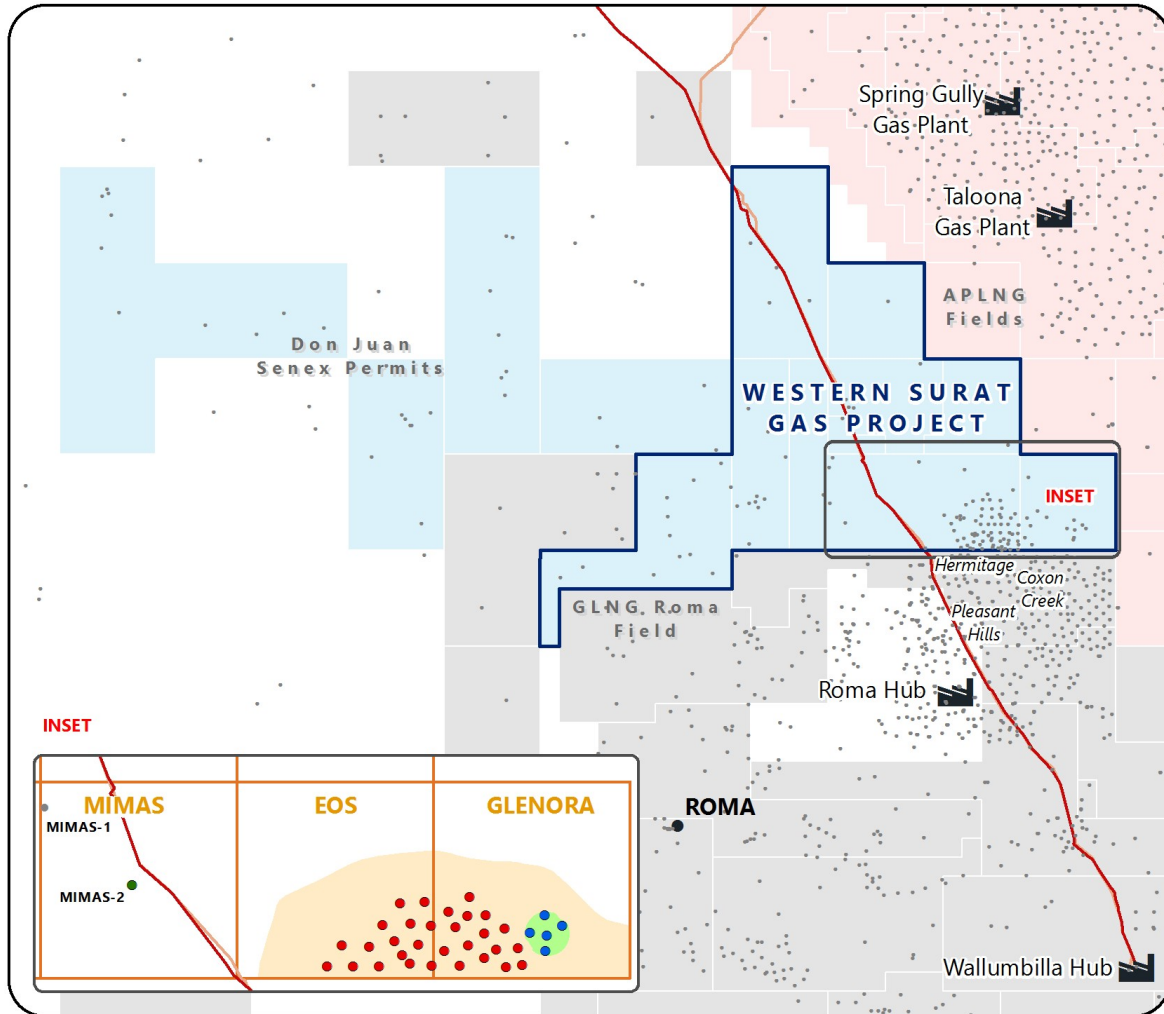
Figure 1: Senex drilling activity for November 2017: Western Surat Gas Project, Surat Basin, Queensland
