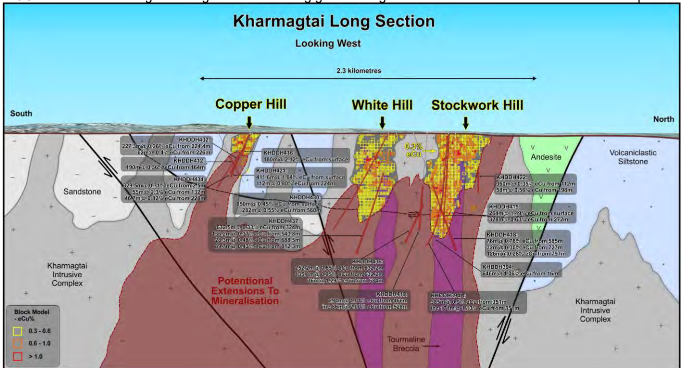
FIGURE 3: Long Section through the three existing deposits showing recent extensions.
