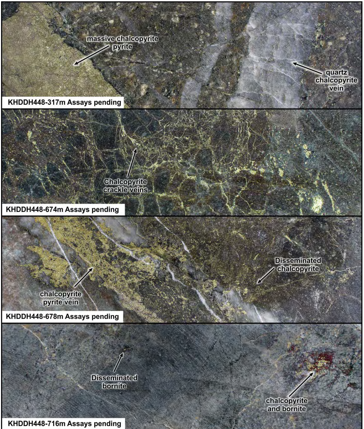
FIGURE 6: Mineralised slab images from KHDDH448, currently drilling. Halved HQ core, the height of each image is 6.35cm
