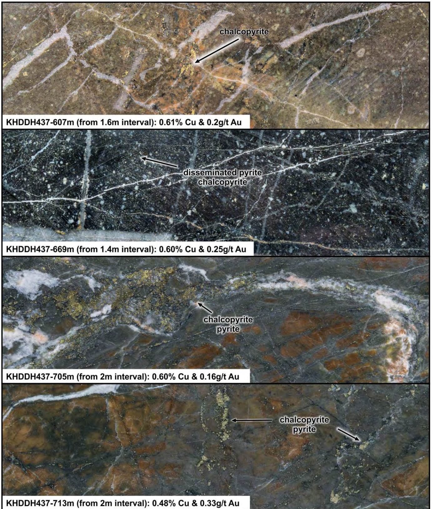
FIGURE 11: Mineralised slab images from KHDDH437. Halved HQ core, the height of each image is 6.35cm
