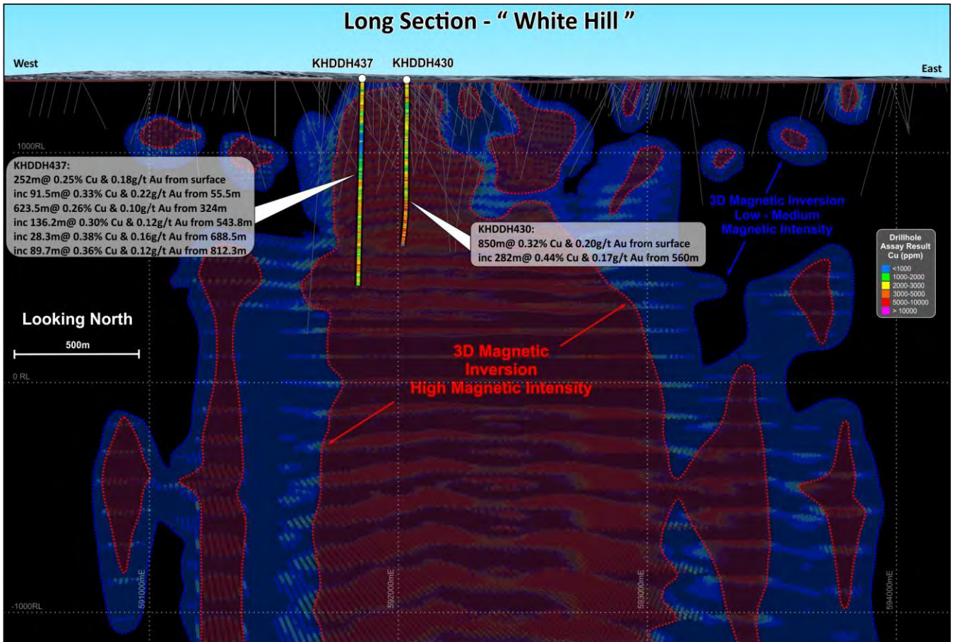
FIGURE 10: Long Section of White Hill showing outline of existing inferred resource, recent significant extensions and 3D magnetic inversion target interpreted to represent the main mineralised porphyry stock.
