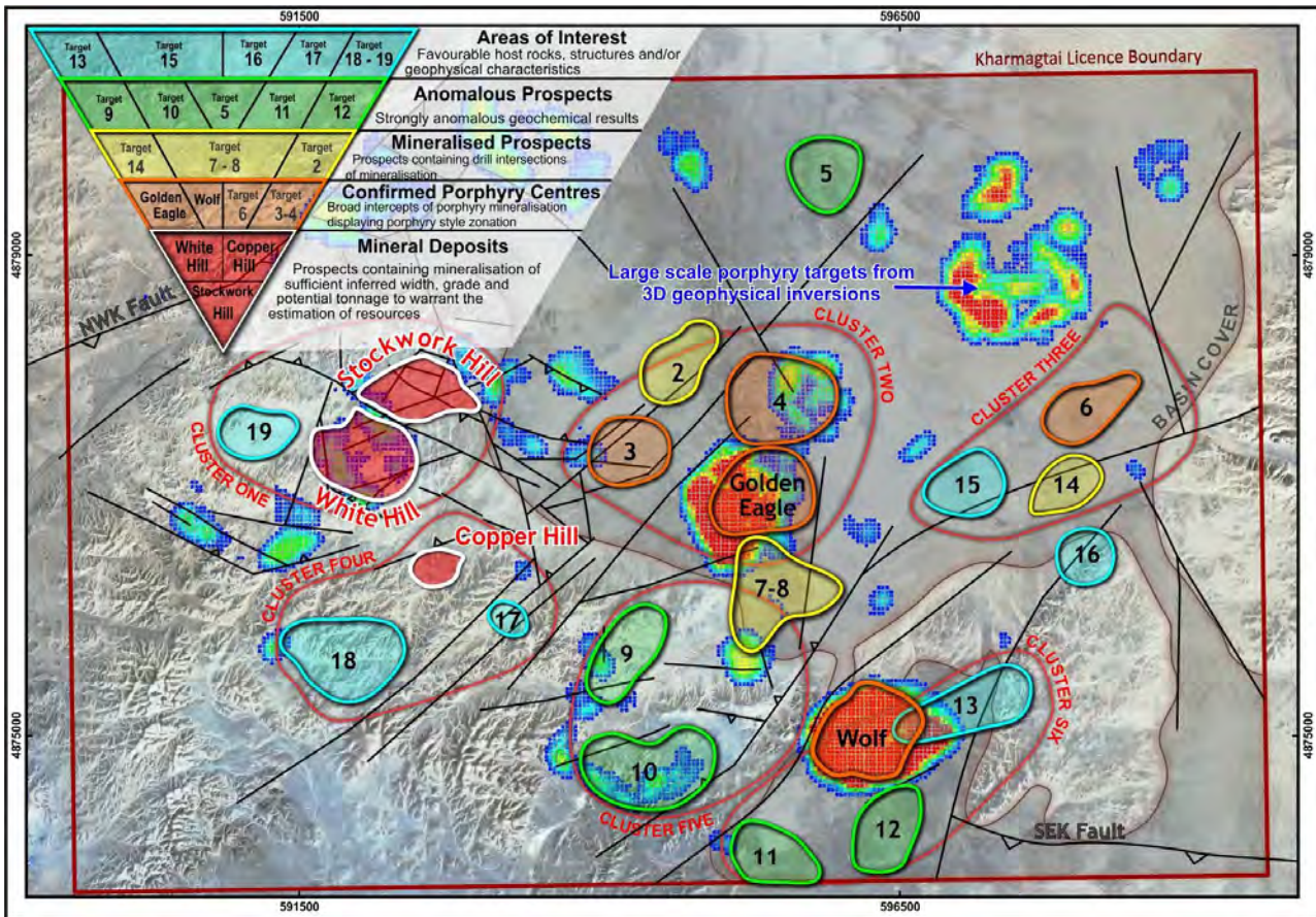
FIGURE 14: The Kharmagtai Mining Licence showing undercover porphyry targets and 3D geophysical inversions map.
