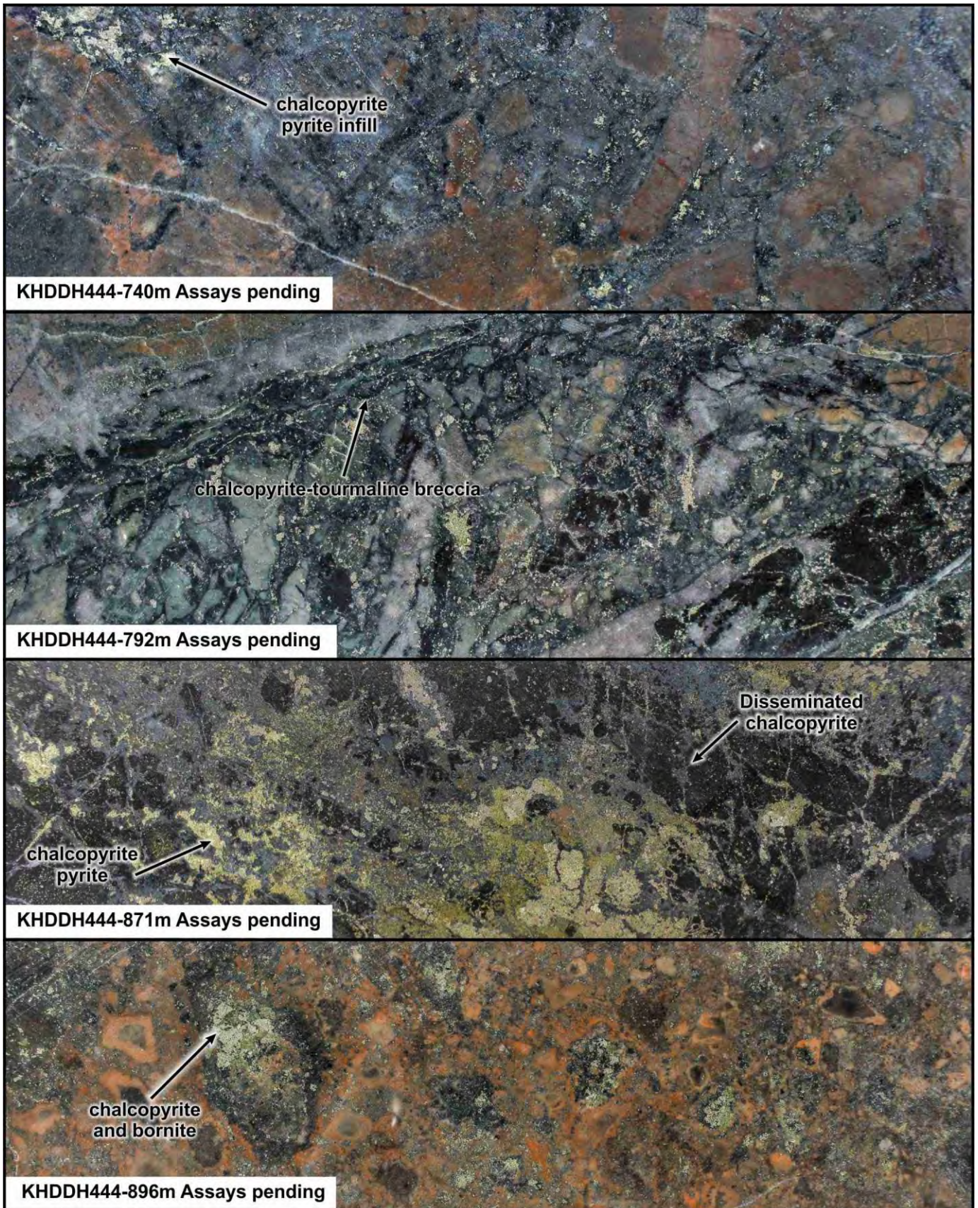
FIGURE 12: Mineralised slab images from KHDDH444 at White Hill, currently drilling. Halved HQ core, the height of each image is 6.35cm
