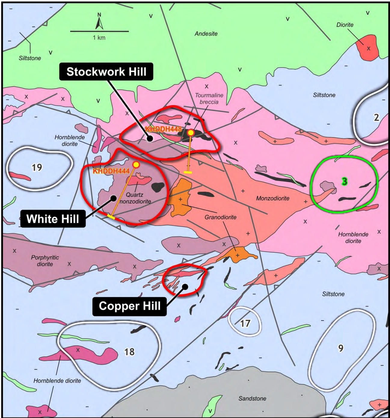
FIGURE 7: Geological map of Stockwork Hill, White Hill and Copper Hill showing two currently drilling hole KHDDH444 and KHDDH448.
