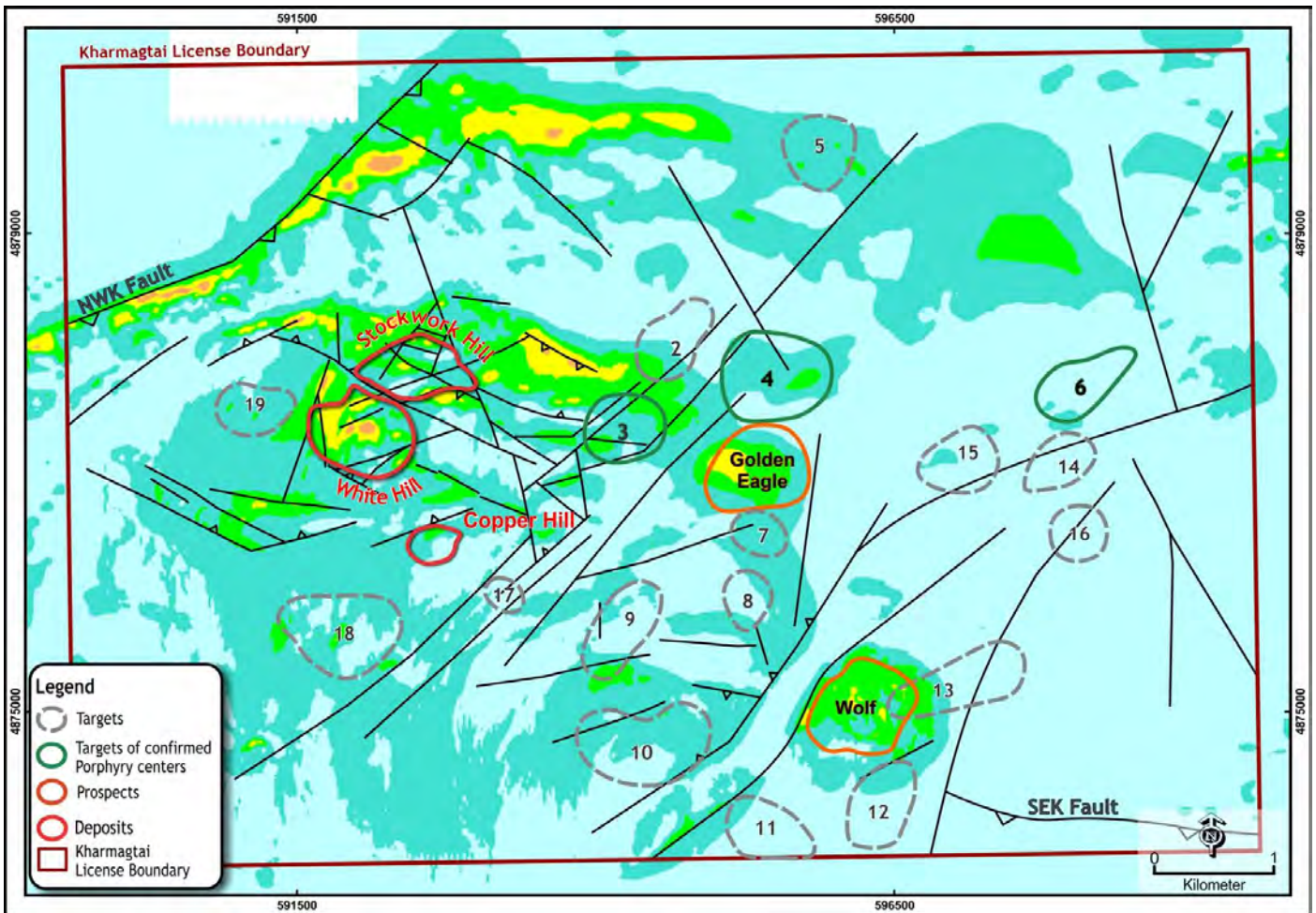
FIGURE 13: Sophisticated reprocessing of the existing ground magnetics focuses on areas where magnetic rotation has occurred. This rotation occurs due to faulting, mineralisation or alteration and helps highlight areas of potential mineralisation. Interestingly, all areas of existing mineralisation are represented and several areas outside known targets are highlighted for follow-up.
