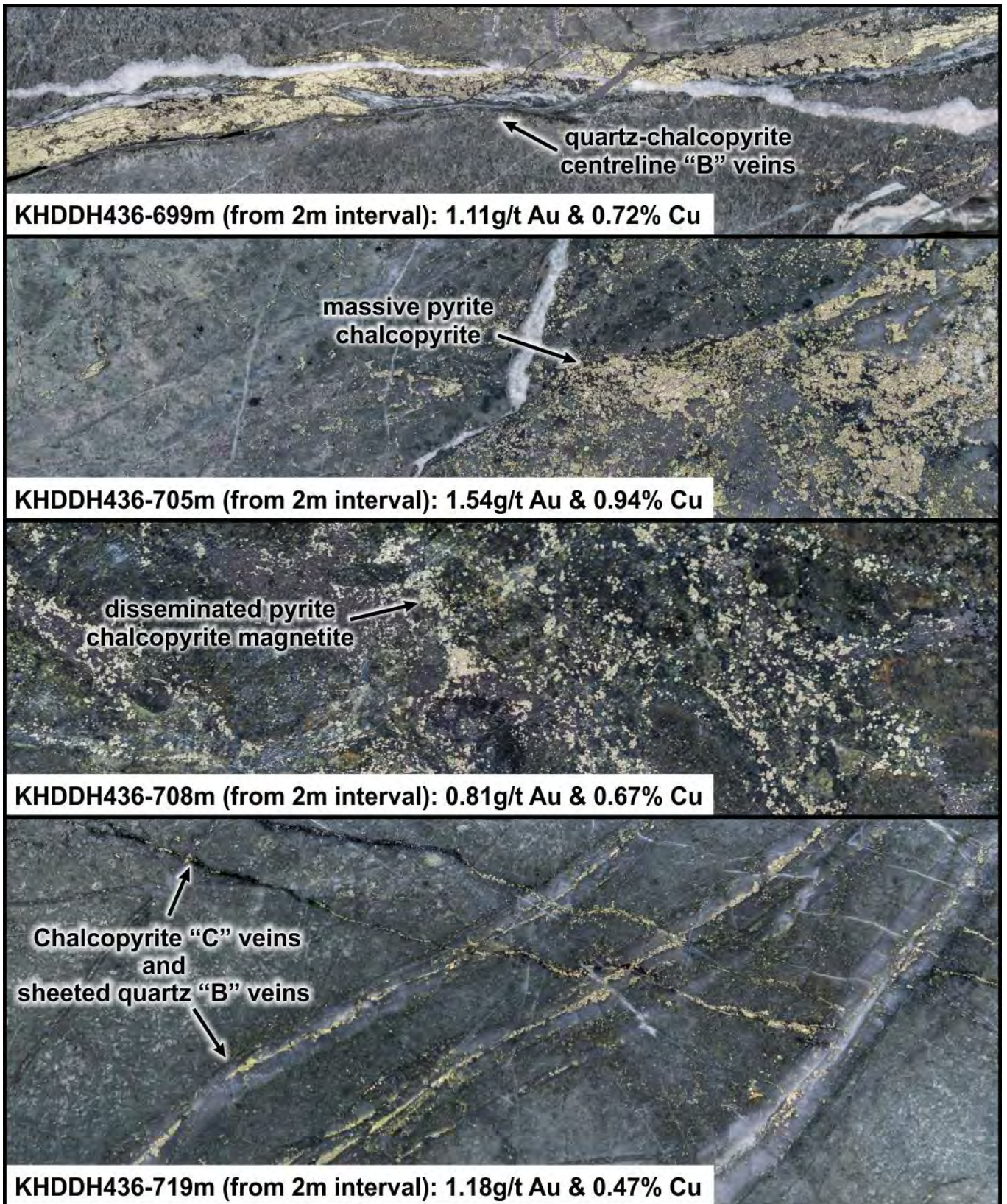
FIGURE 5: Mineralised slab images from KHDDH436. Halved HQ core, the height of each image is 6.35cm
