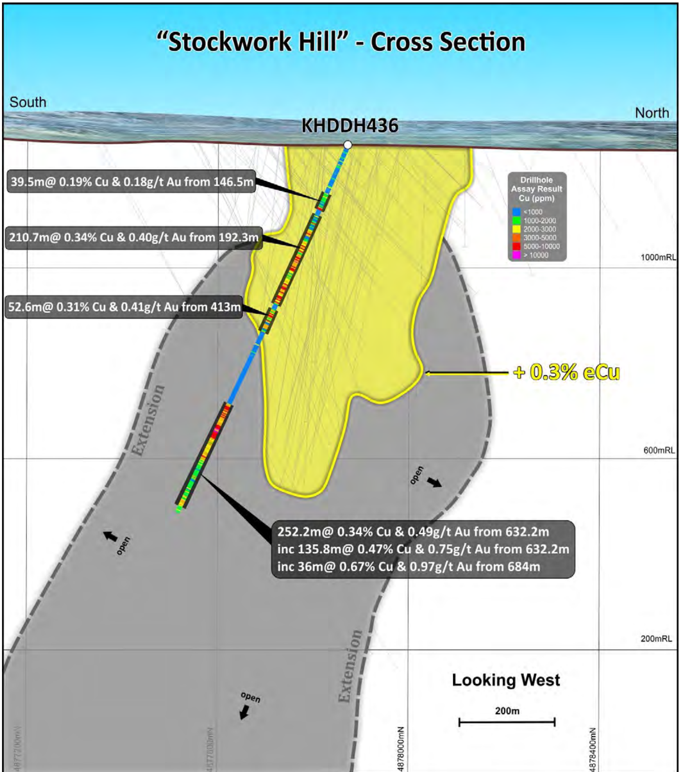
FIGURE 4: Cross section through Stockwork Hill showing outline of existing inferred resource and recent significant extensions.
