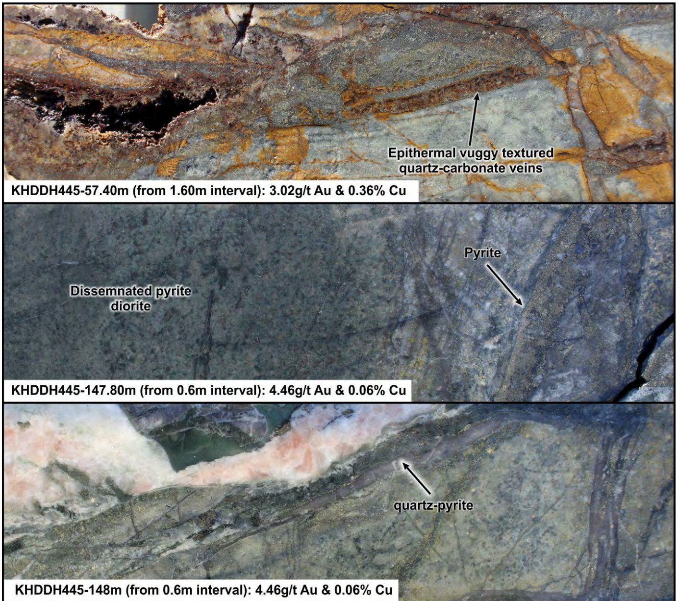
FIGURE 15: Mineralised slab images from KHDDH445. Halved HQ core, the height of each image is 6.35cm
