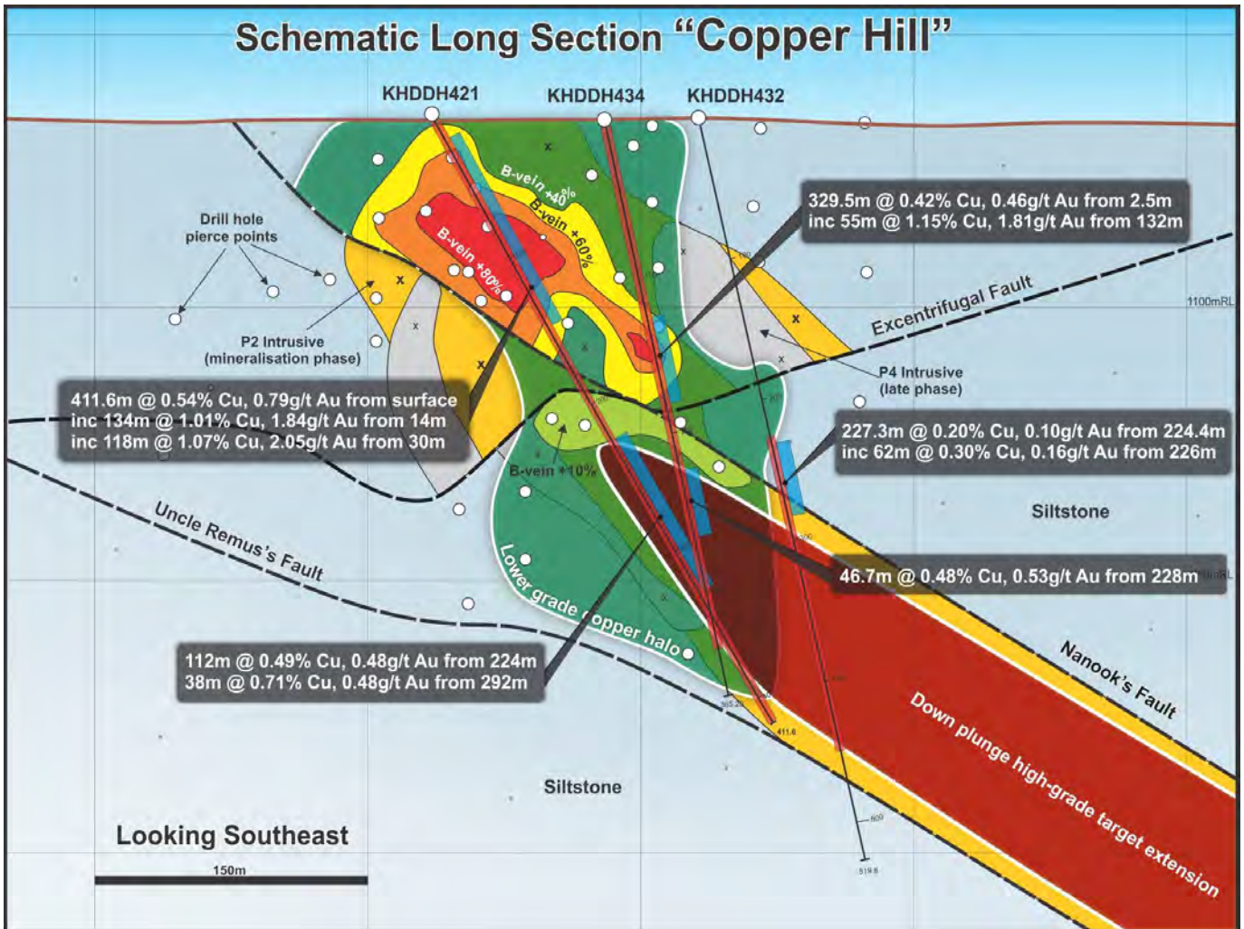
FIGURE 8: Schematic long section through Copper Hill showing drill holes KHDDH432 and KHDDH434 and the down-plunge target zone. Recent drill holes are shown in their entirety rather than as pierce points on the section and these holes therefore project from behind to in front of the schematic section.
