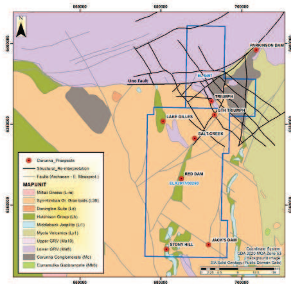
Figure 5: Revised structural interpretation, prospects and regional geology (Blundell, 2017).
