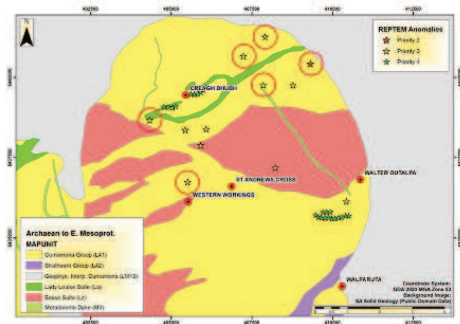
Figure 12: Prioritised EM anomalies (Blundell, 2018).
