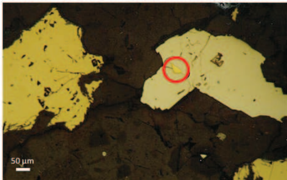
Figure 13: Photomicrograph from Walparuta Cu-Au Mine. Yellow Mineral = Chalcopryrite, White Mineral = Pyrite and Red Circle = Au (25x50µm) (Pontifex, 1990).
