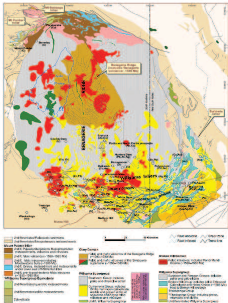
Figure 7: Curnamona Province solid geology interpretation (Burtt et. al., 2004).
