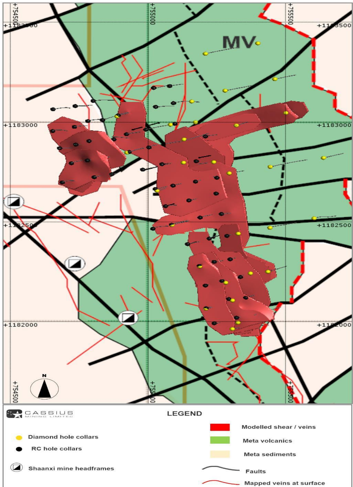
Figure 11: Plan view showing outline of the mineralised shear-veins
