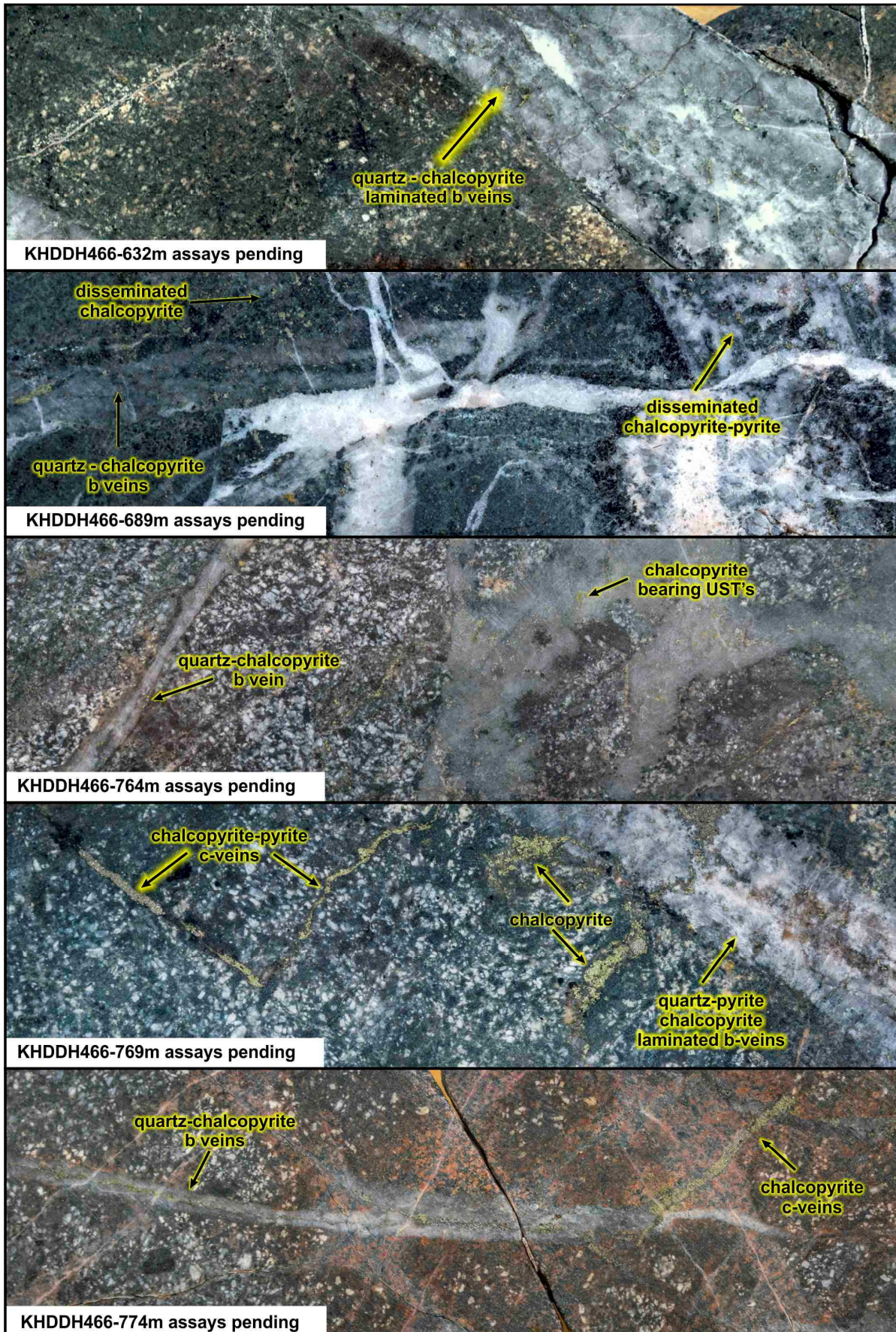
FIGURE 5: Mineralised slab images from KHDDH466. Halved NQ core, the height of each image is 4.7cm.
