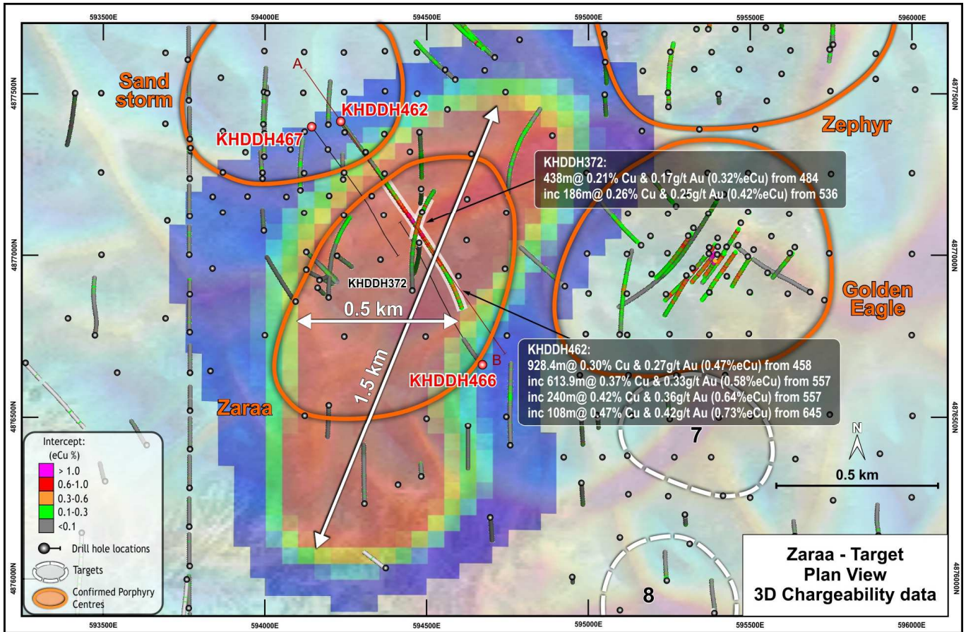
FIGURE 3: Plan view of Zaraa, showing returned assays and previous drilling over 3D IP data.
