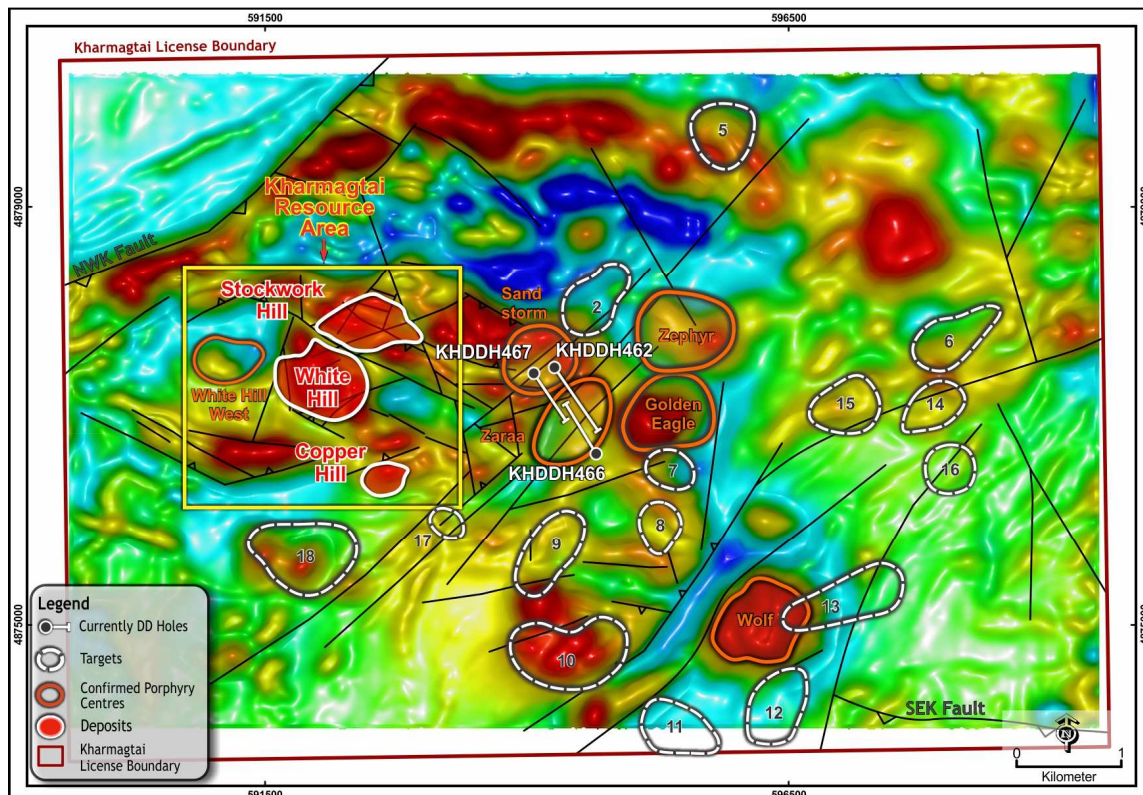
FIGURE 2: The Kharmagtai District showing ground magnetic data and location of the Kharmagtai Deposit (Stockwork Hill, White Hill, Copper Hill), porphyry centres, targets and location of Zaraa and current drilling.
