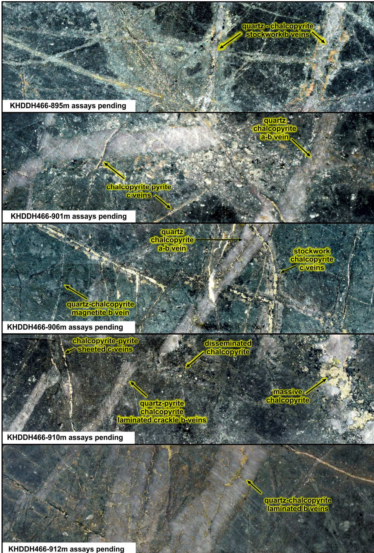
FIGURE 3: Mineralised slab images from KHDDH466. Halved NQ core, the height of each image is 4.7cm.
