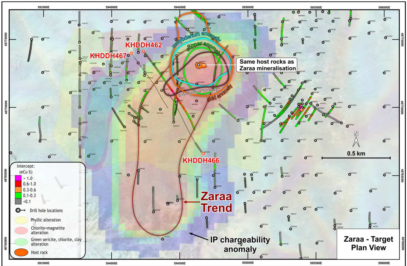
FIGURE 5: Projected location of the Zaraa discovery at the basement surface.
