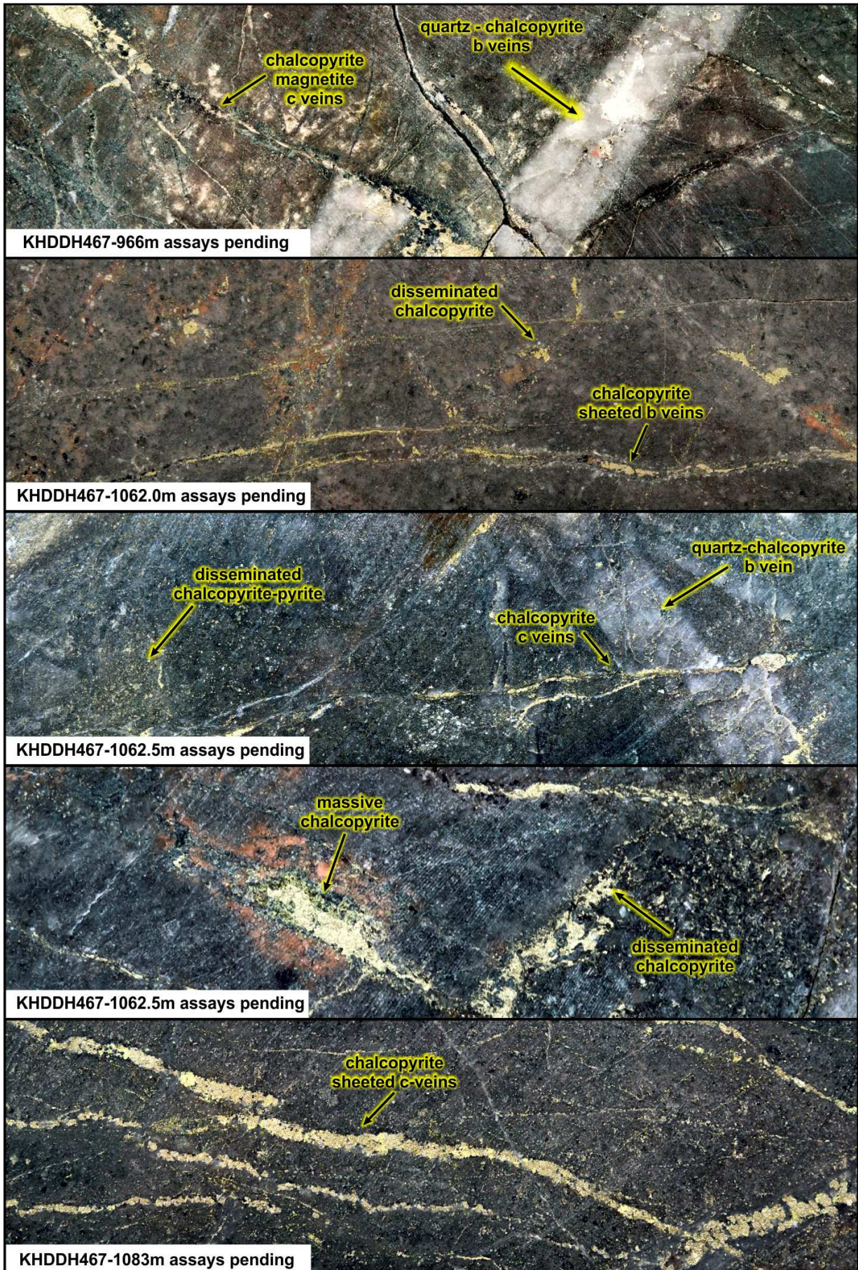
FIGURE 4: Mineralised slab images from KHDDH467. Halved HQ core, the height of each image is 6.35cm.
