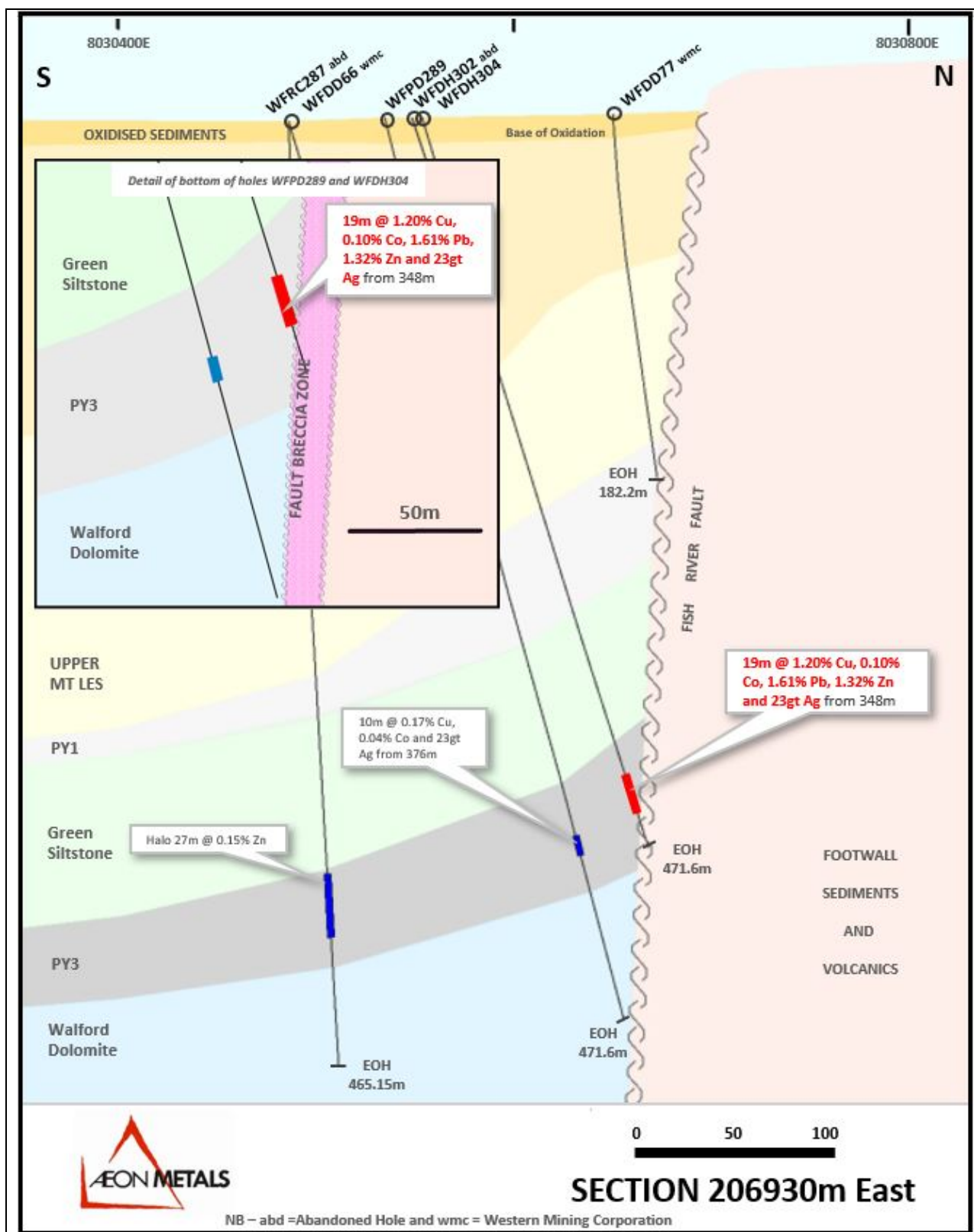
Figure 1 Section showing latest assay results from hole WFDH304 on section 206930E.
