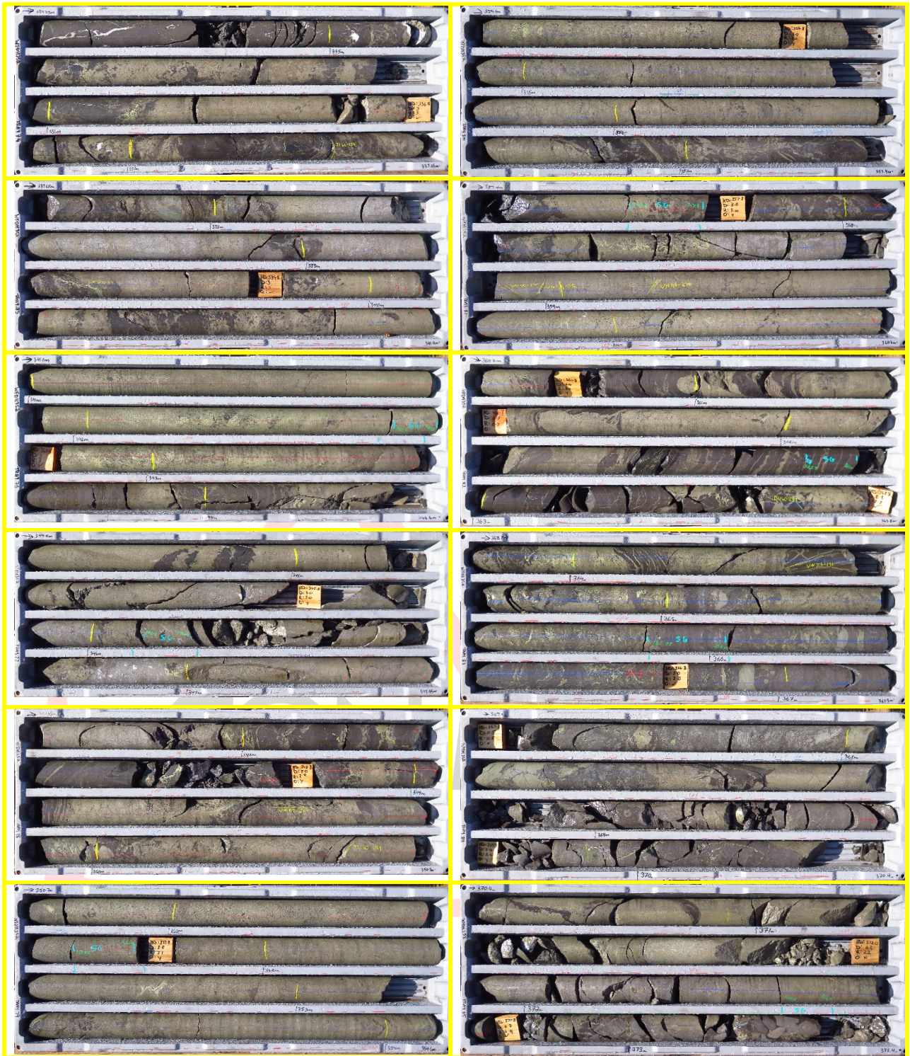
Figure 1 Photos of core from the 42m interval starting at 332m and going to 374m in hole WFDH352 showing massive to semi-massive chalcopyrite and pyrite mineralisation.
