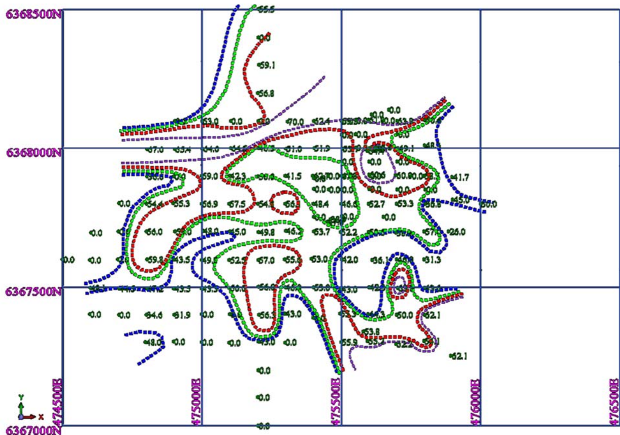
Minus 45µm Micron Average Hole Recovery Contour Map
