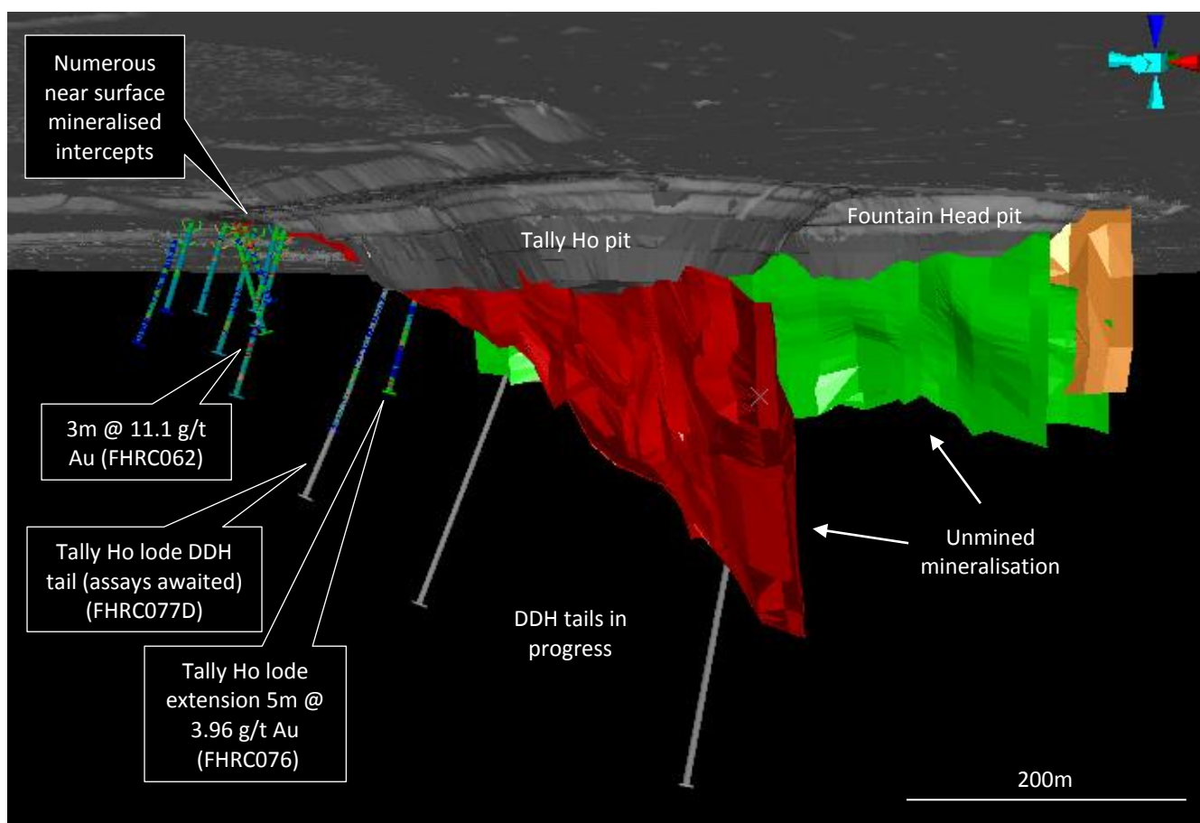
Figure 2: Isometric view of mineralisation (modelled from historic drilling) looking approximately north-east from below surface showing Tally Ho lode (red), Fountain Head lodes (green/orange), and PNX drill holes. The limited extent of historic mining is also shown.
