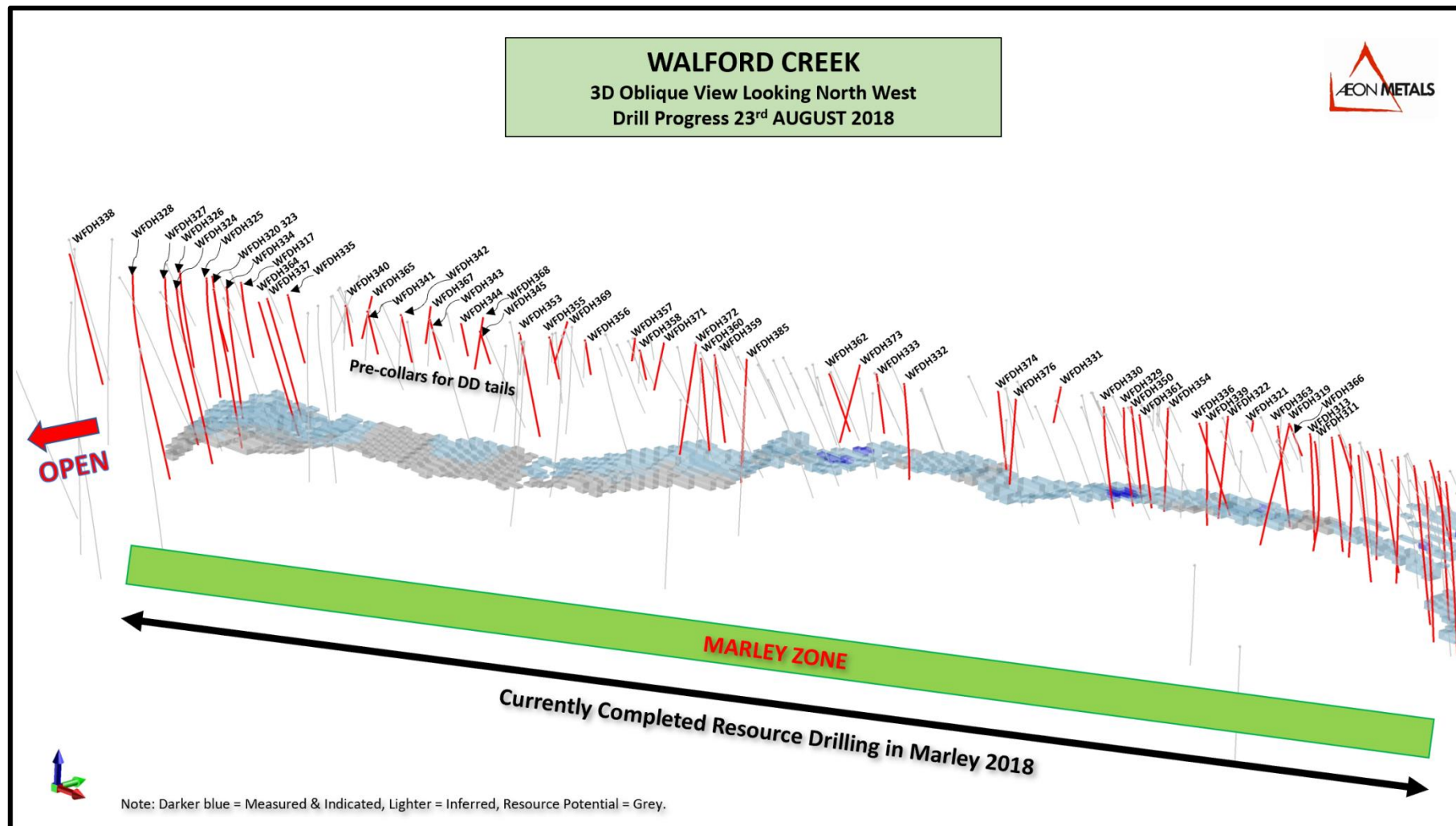
Figure 2: 3D oblique view showing 2018 Marley Resource drilling.
