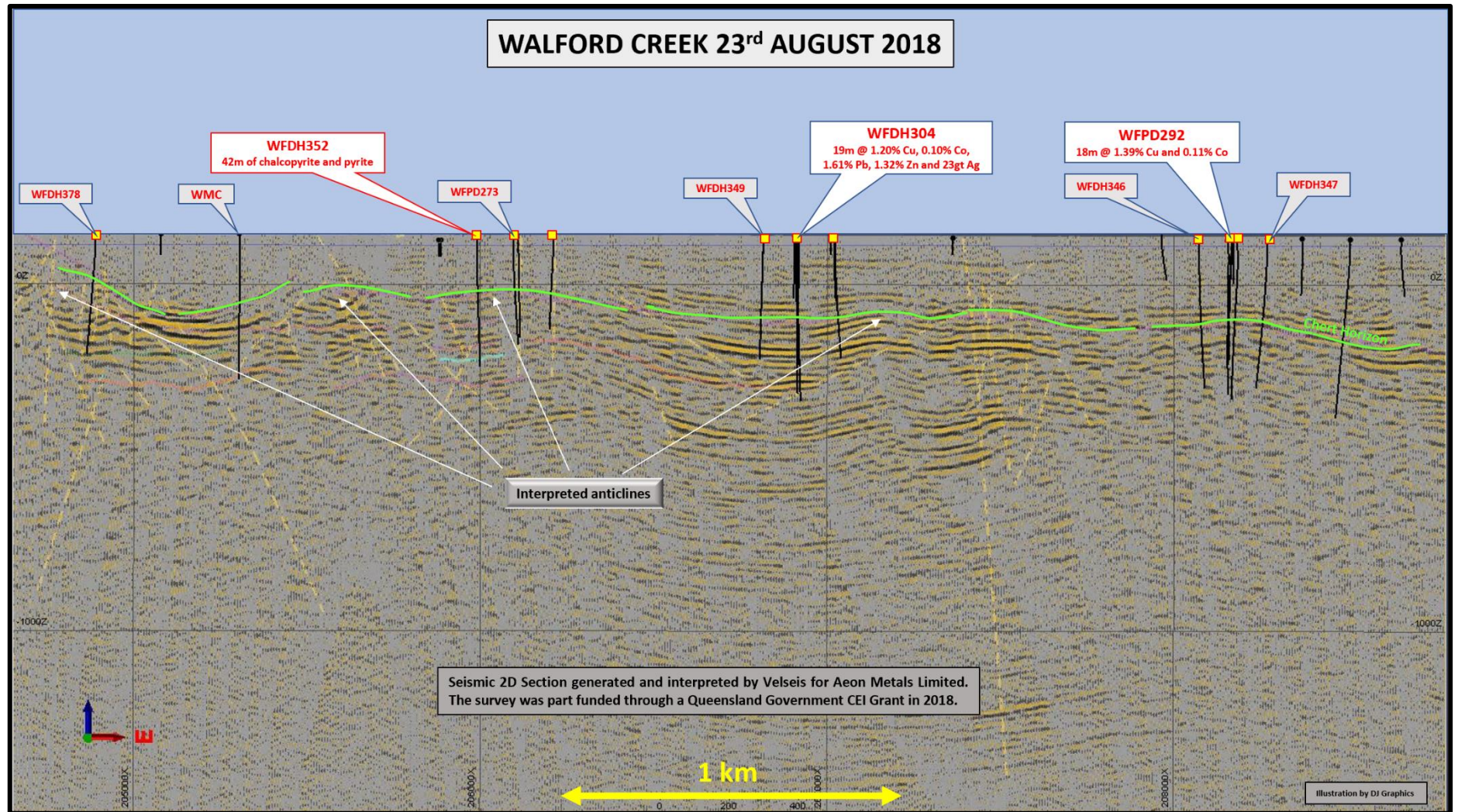
Figure 3: Long Section view of east-west 2D seismic line showing Velseis interpretation with significant exploration drilling undertaken by Aeon in 2018. Shows location of hole WFDH352 which intersected over 40m of strong chalcopyrite mineralisation in what is now recognised as an anticlinal feature in the seismic data.
