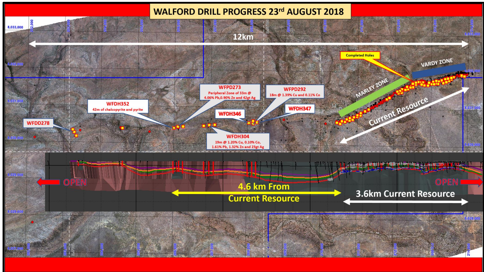
Figure 4: Walford Creek Project. Plan and scaled long section showing current resource, interpreted stratigraphy along the strike of the Fish River Fault and indicative planned initial holes.
