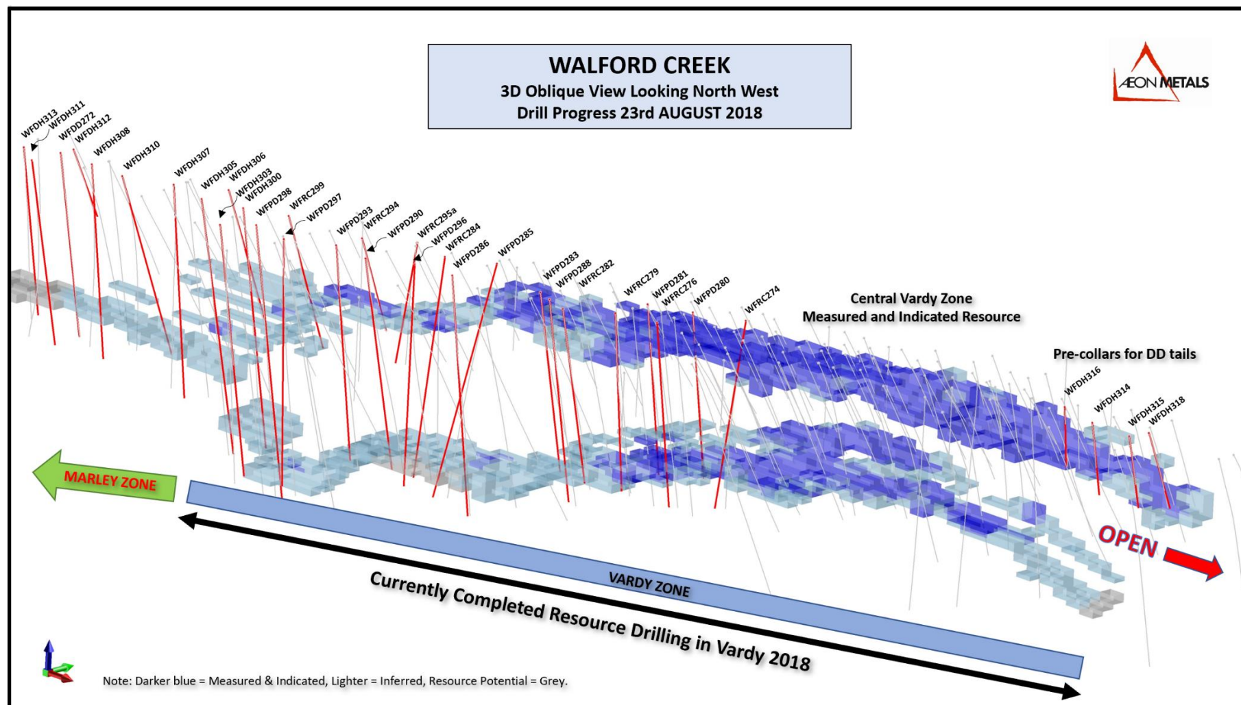
Figure 1: 3D oblique view showing 2018 Vardy Resource drilling.
