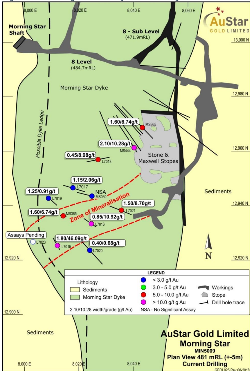
Figure 1. Plan Showing Pierce Points of Current Drill Program Stones - Maxwells
