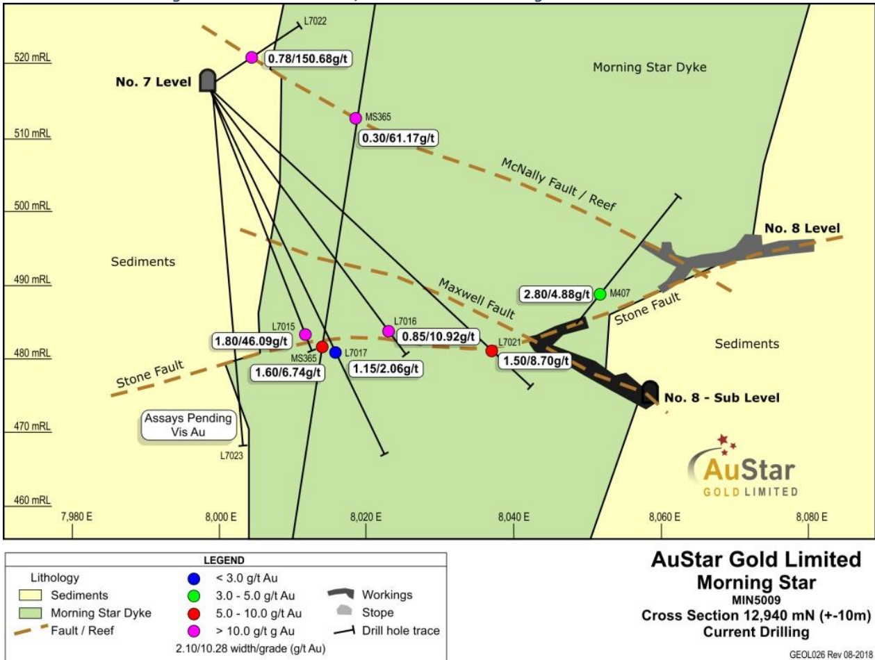
Figure 2. Cross Section at 1,930mN Current Drill Program Stones – Maxwells.
