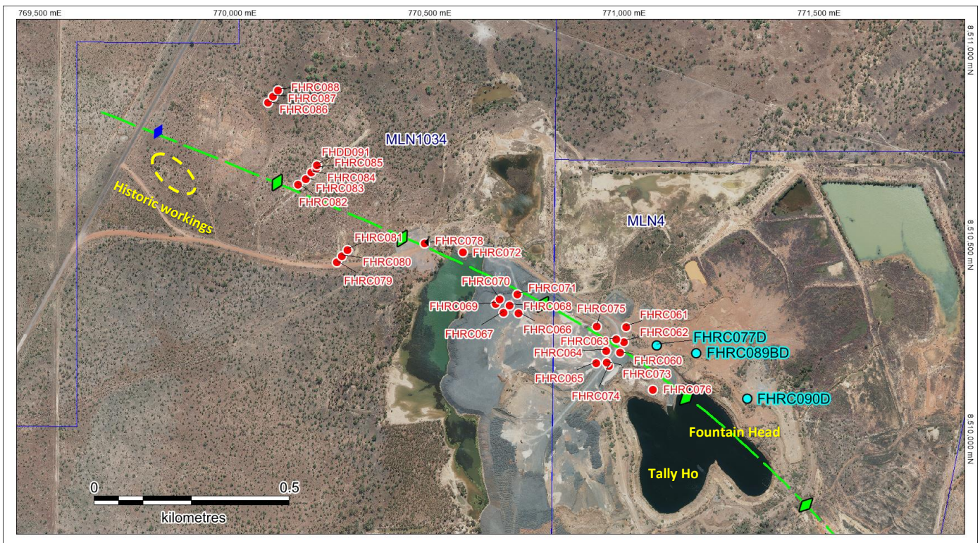
Figure 2: Historic Fountain Head and TallyHo mining area and location of PNX drill holes. Red = assays reported, Blue = diamond holes awaiting assays, Green line is the Fountain Head Anticline thought to control mineralisation
