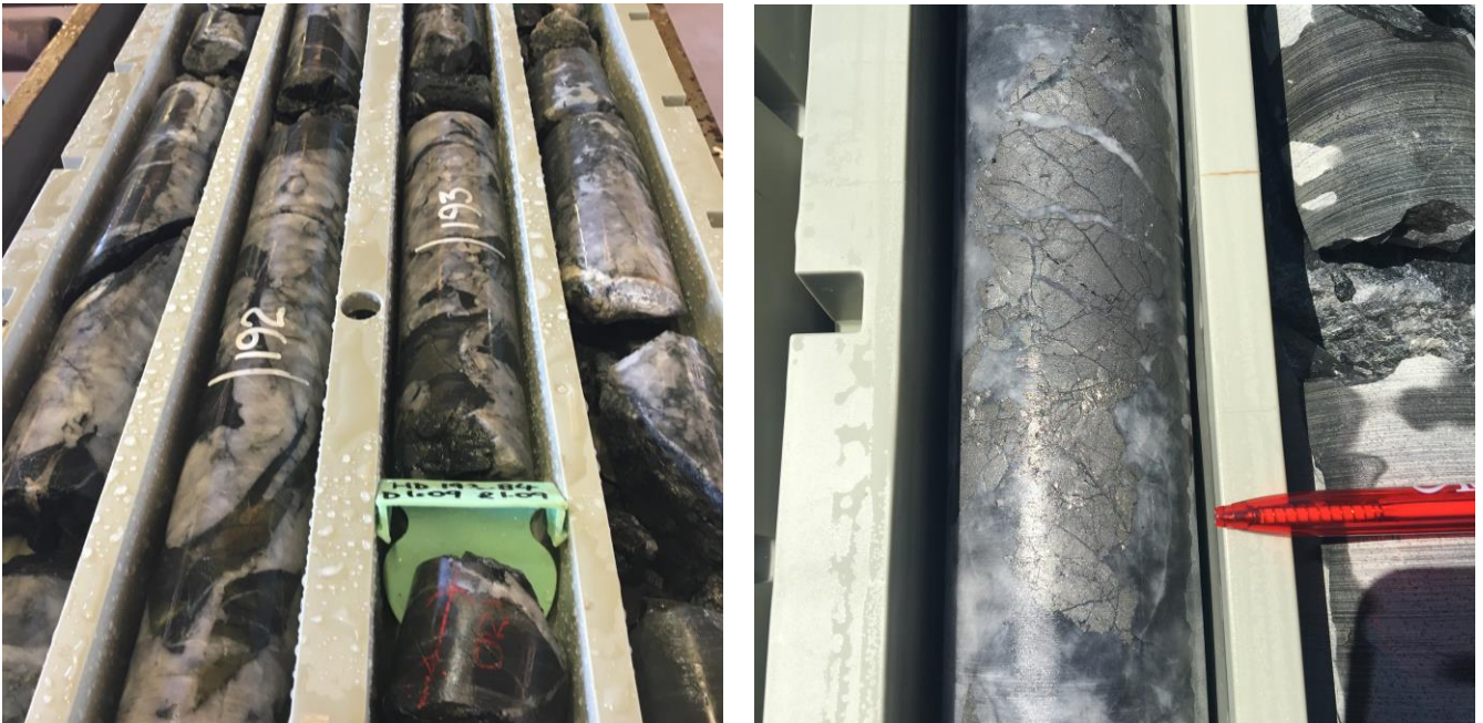
Figure 1: FHRC077D (left) from 191m showing mineralised zone, and FHRC090D (right) at 375 metres showing massive arsenopyrite within quartz, both holes drilled to extend the Tally Ho lode
