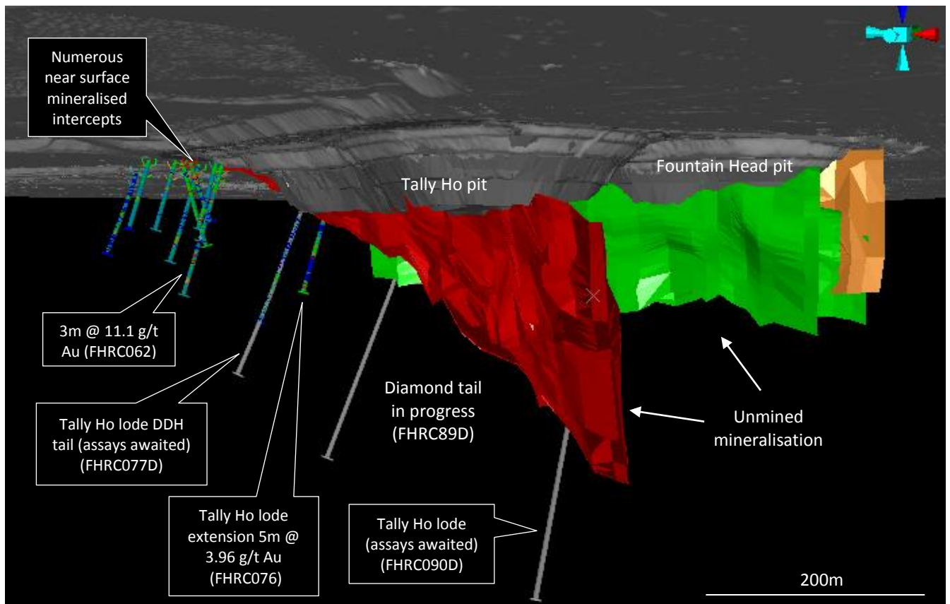
Figure 3: Isometric view of mineralisation (modelled from historic drilling) looking approximately north-east from below surface showing Tally Ho lode (red), Fountain Head lodes (green/orange), and PNX drill holes. The limited extent of historic mining is also shown.
