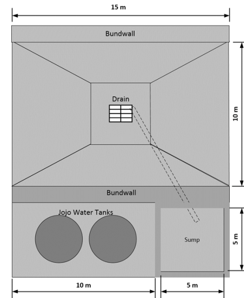
Wash Bay
