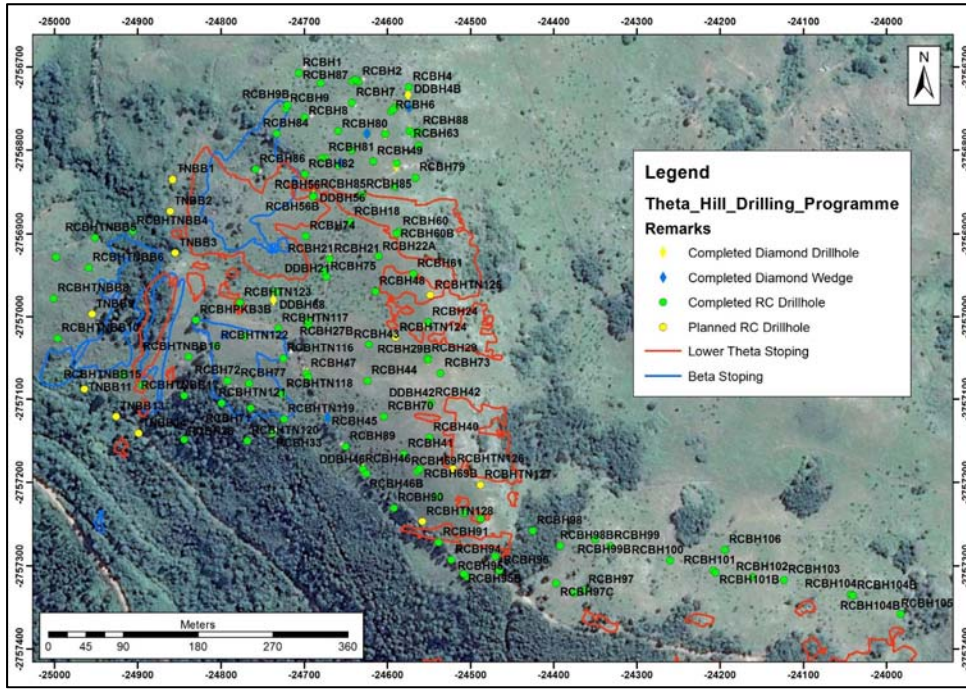
Figure 2: Updated Distribution of Boreholes at Theta Hill North
