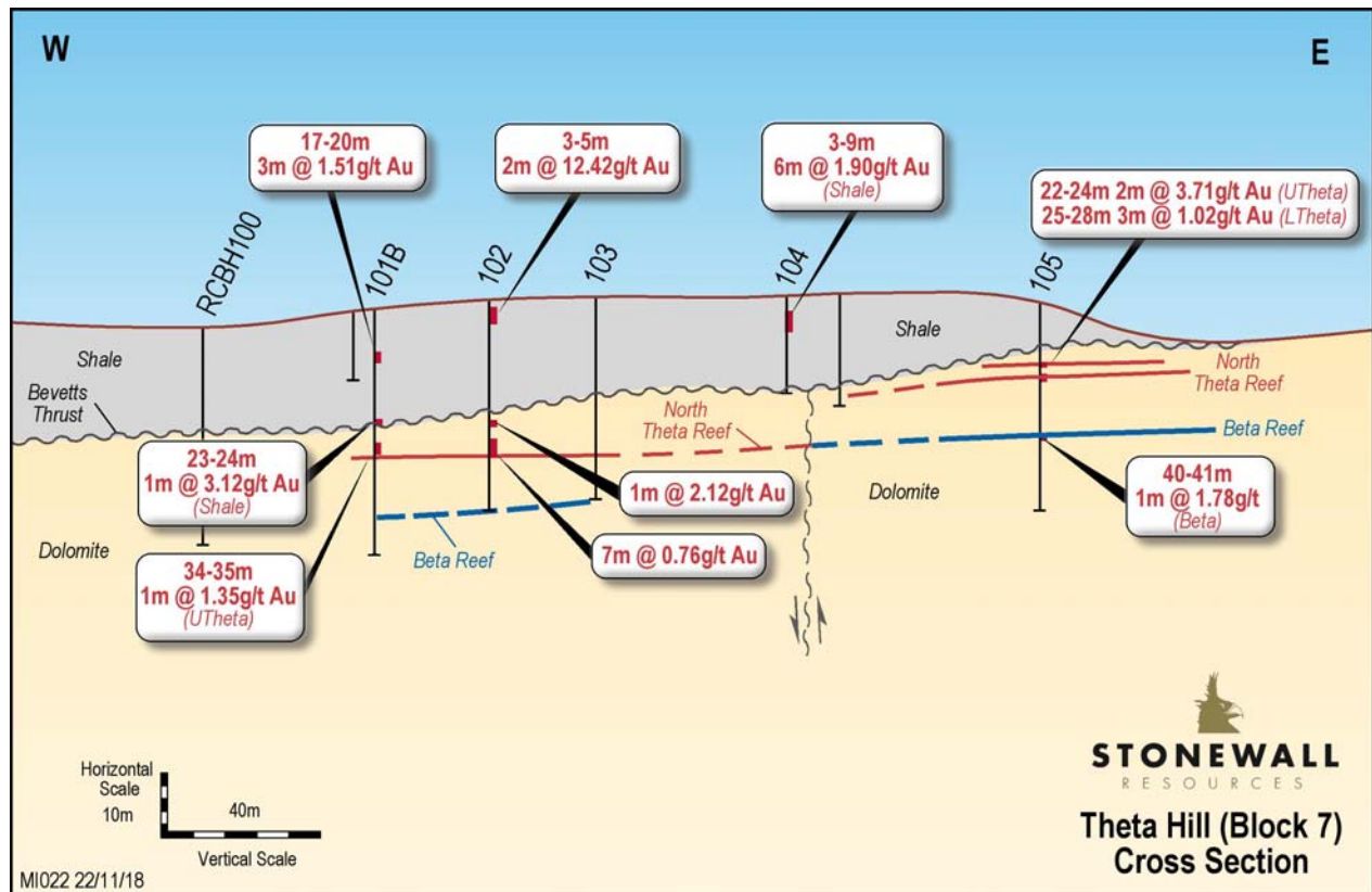
Figure 4: A West-East cross section of Theta Hill Block 7 drill interpretations
