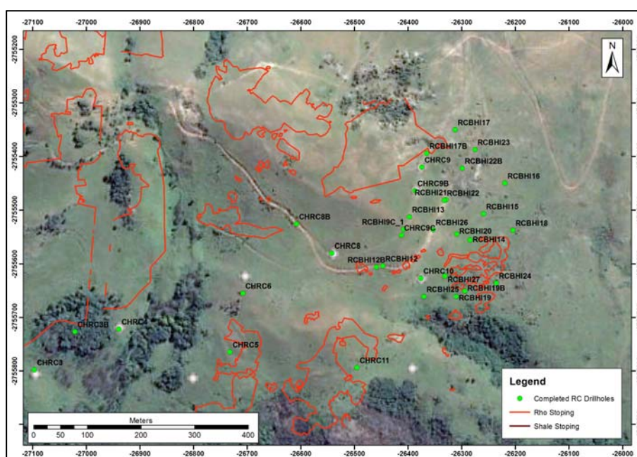
Figure 5: Distribution of RC drilling at Columbia Hill (Iota Mine workings)
