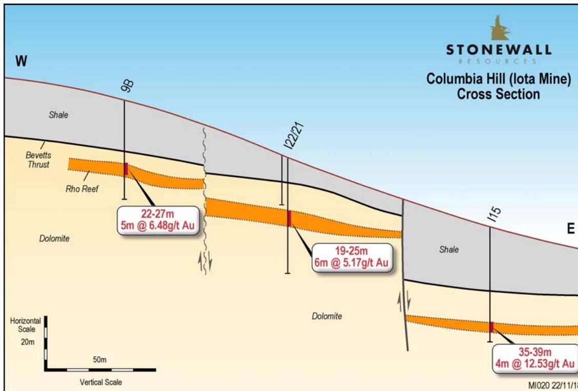
Figure 6: Columbia Hill (Iota Mine) Cross Section with Rho Reef intersections
