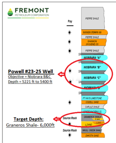
Figure 2: The JW Powell #23-25 well is targeting production from the Niobrara Formation B and C Benches
