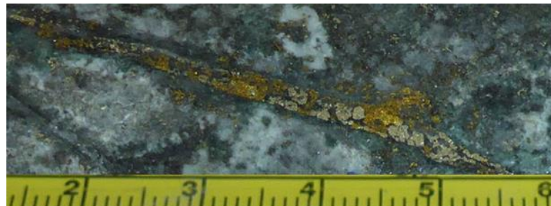
Fig: MCD002, 129.18 m - Molybdenite selvage on quartz. B-type veins are particularly distinctive of porphyry copper-gold systems (scale: cm)
