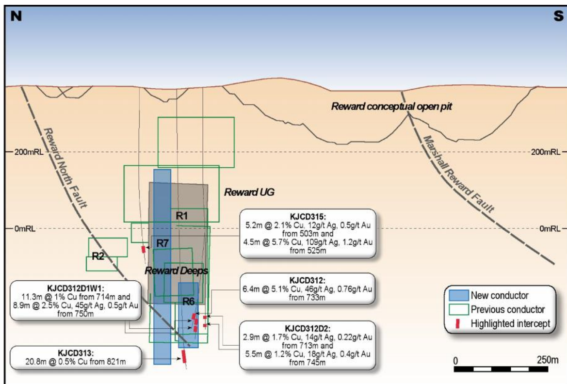
Figure 2: Longitudinal section of the existing and new conductors at Reward Deepes with assays of KJCD312, KJCD312D1W1 and KJCD312D2, KJCD313 and KJCD315.
