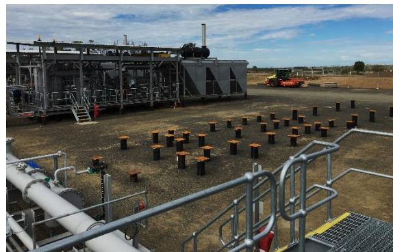
Compression equipment and piles for expansion (foreground)
