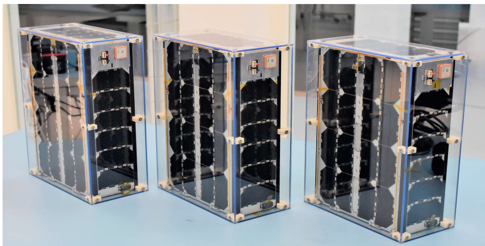
Three of Kleos' Scouting Mission four satellites transport ready (Satellite four remained available for algorithm development at time of photo)
