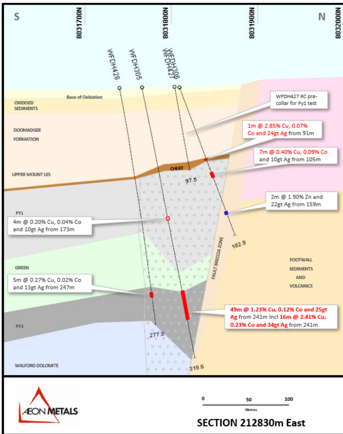
Figure 5 Section 212830E shows hole WFDH427 and WFDH428
