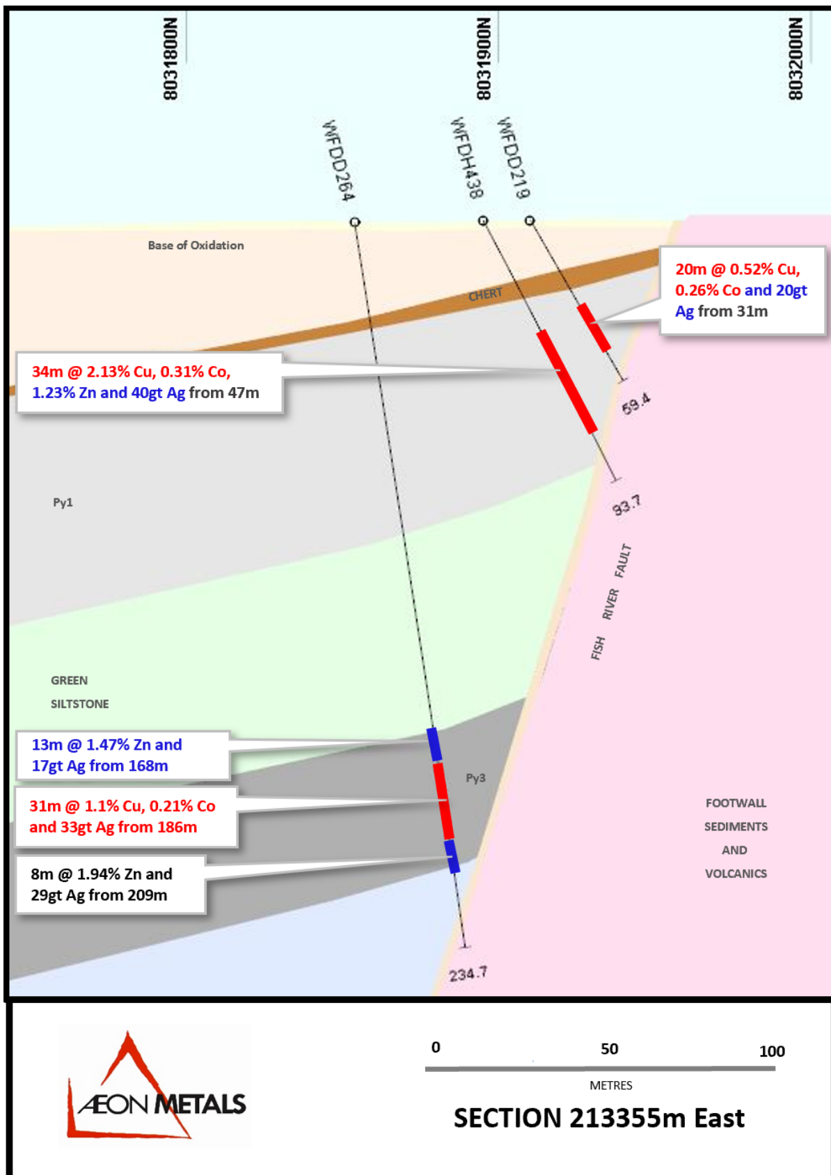
Figure 2 Section 213355E shows recent hole WFDH438.
