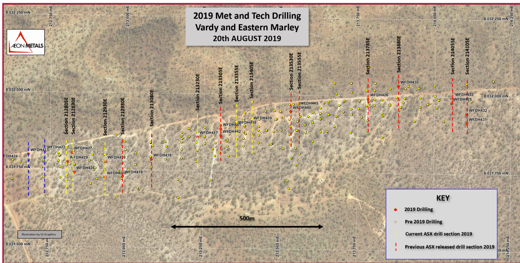
Figure 7 Shows details of sections within Vardy for current ASX release
