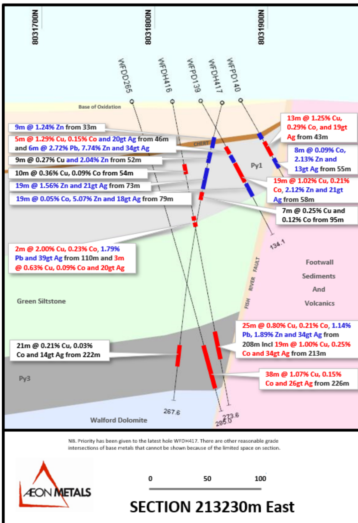
Figure 3 Section 213230E shows recent hole WFDH417
