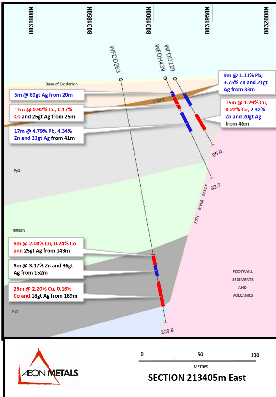
Figure 1 Section 213405E shows recent holes WFDH439
