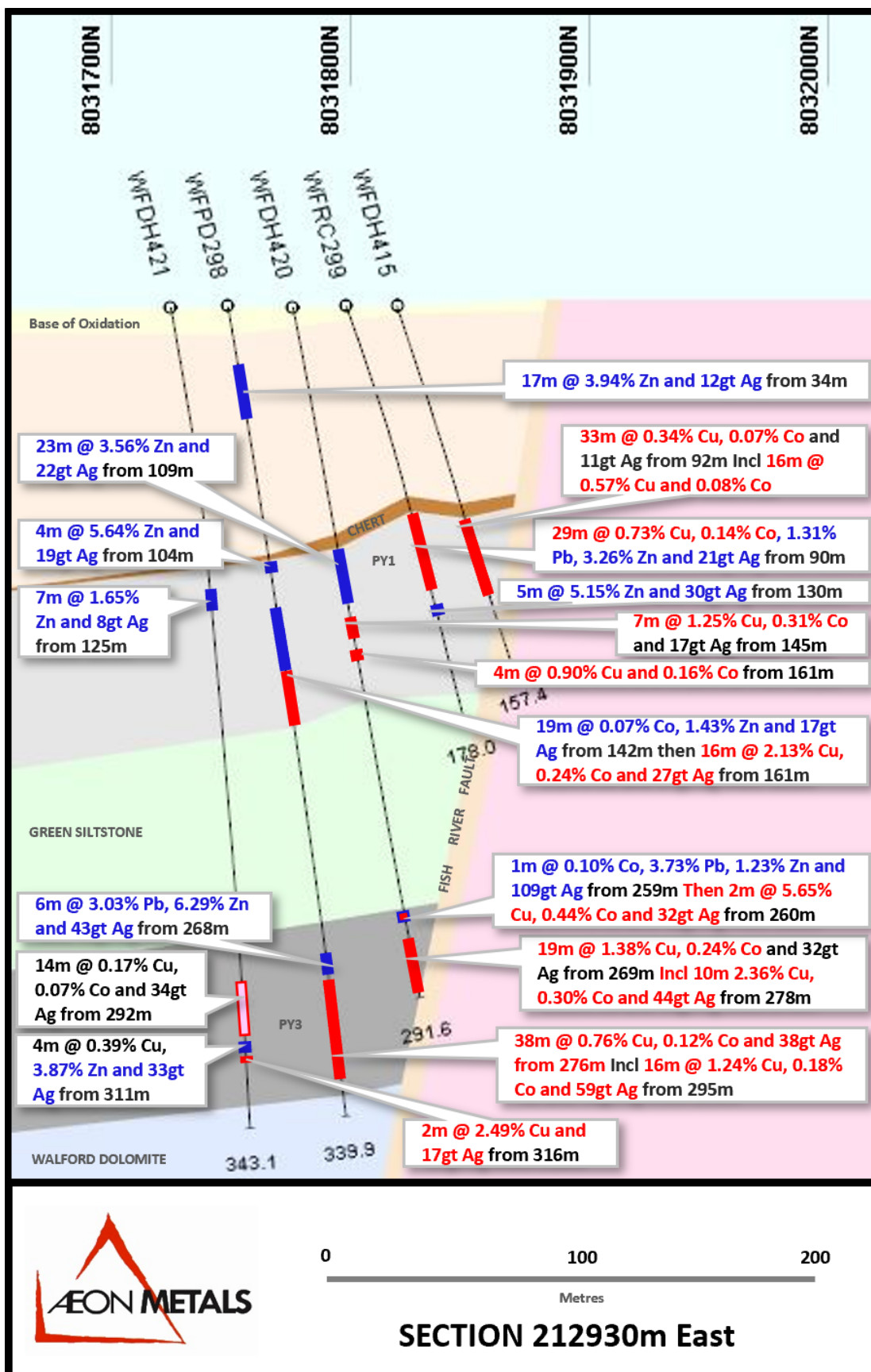
Figure 4 Section 212930E shows recent hole WFDH420 and WFDH421
