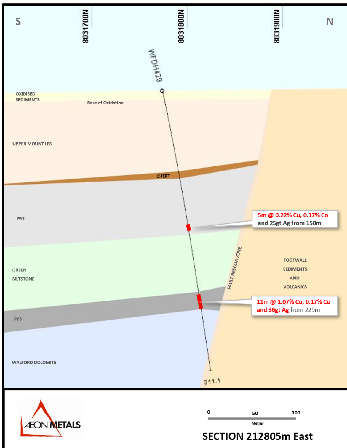
Figure 6 Section 212805E showing hole WFDH429
