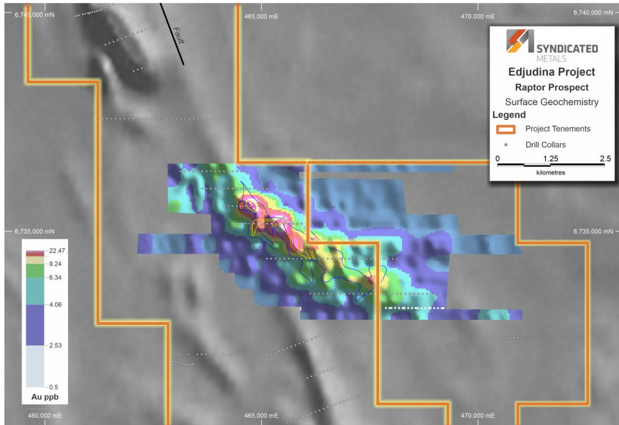
Figure 6: Raptor Prospect surface geochemistry with historic AC drill collars 1
