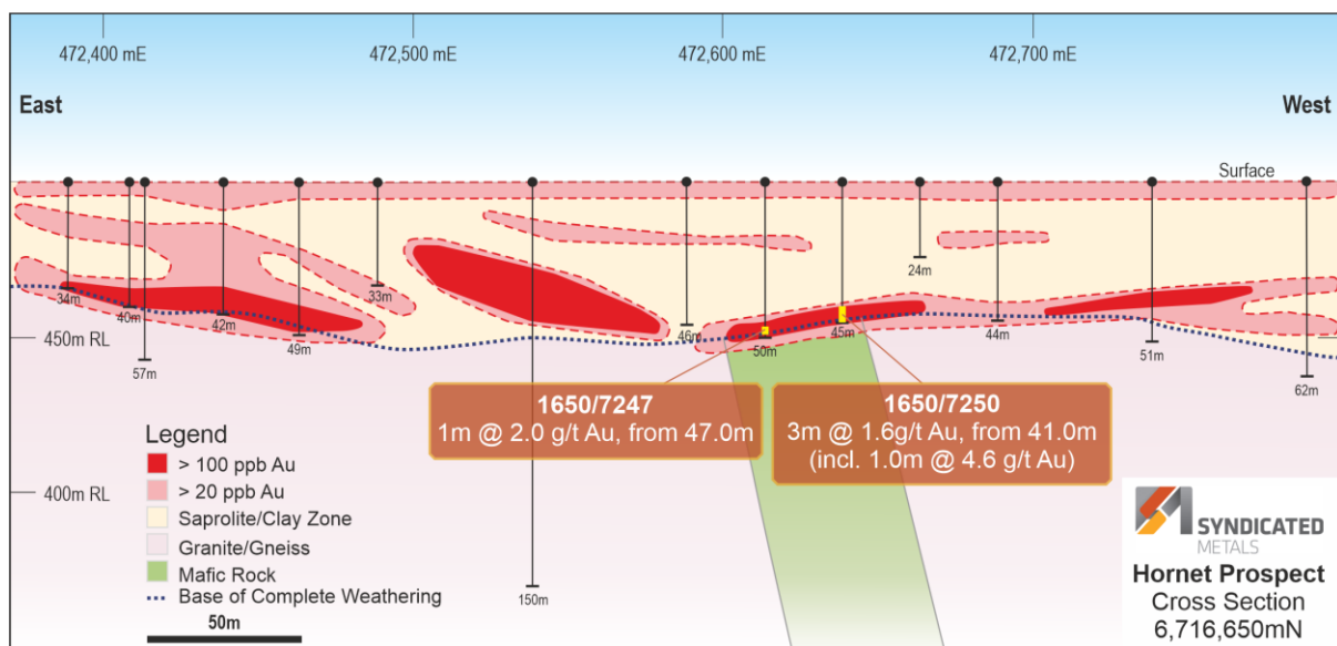
Figure 3: Hornet Prospect section 6,716,650mN (+/- 50m) 1
