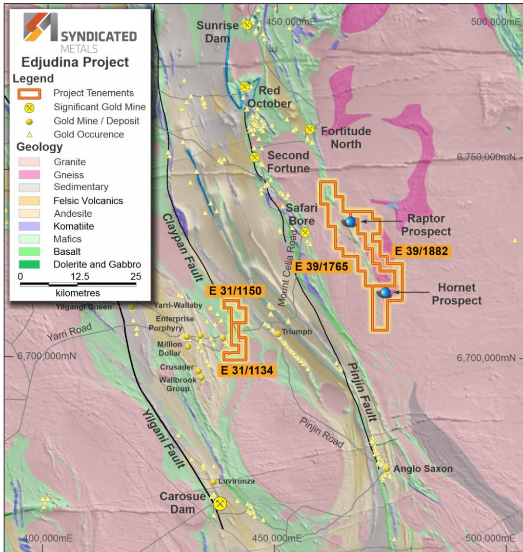
Figure 1: Regional location of the Edjudina Gold Project
