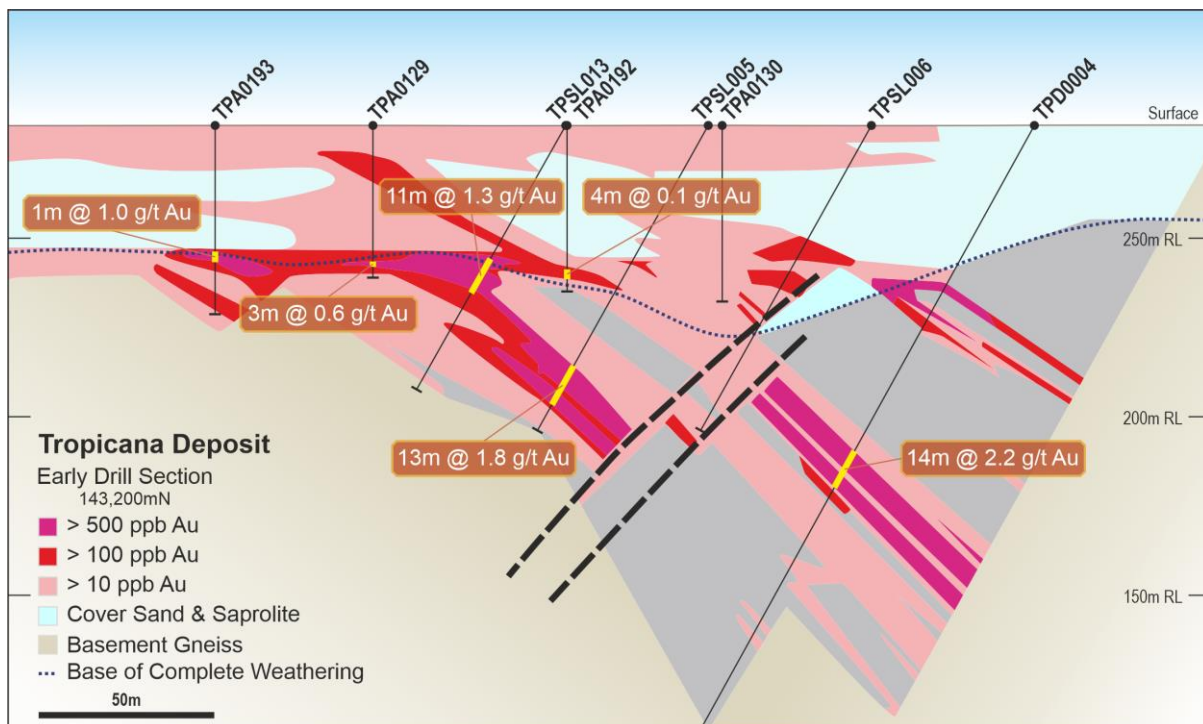
Figure 5: Tropicana Deposit – Early Drill Section 143,200mN 2
