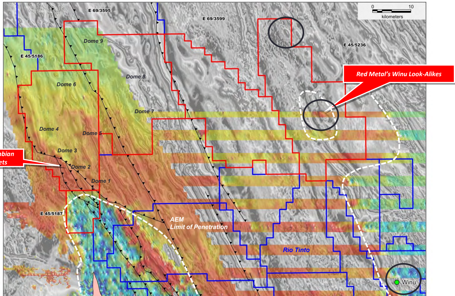
AEM Conductivity Depth Slice 200-250m on Tilt Residual Magnetic Image
