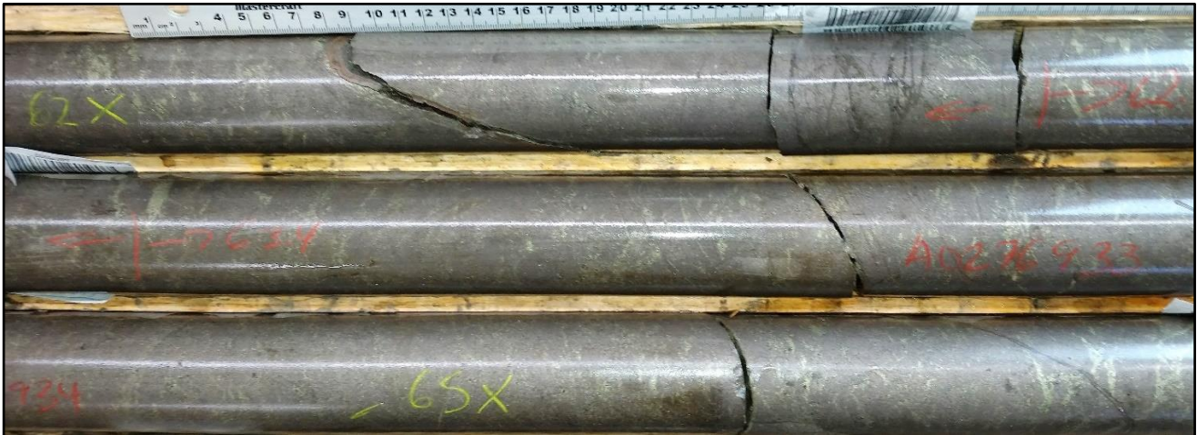
Figure 5: ZA-19-05 massive pyrrhotite with 5-10% visual chalcopyrite at 65m downhole. Interval 62.4 to 65.4m assayed 3.0m at 2.43% Ni, 2.95% Cu, 2.6g/t PGE and 5g/t Ag.
