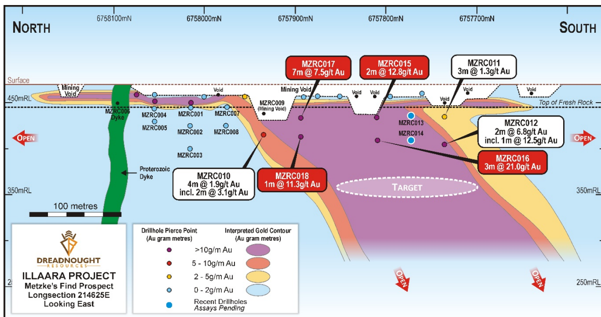
Figure 1: Long section of Metzke's Find showing the extent of shallow historic workings, drilling and the results of recent drilling by Dreadnought – assays pending in blue.
