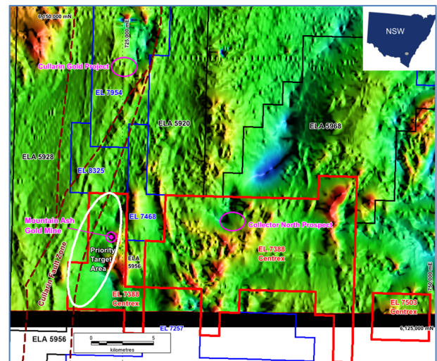
Regional TMI image showing Centrex's exploration licences 7388 and 7503 in red with the priority target areas near the Mountain Ash Gold Mine and the Collector North Prospect.
