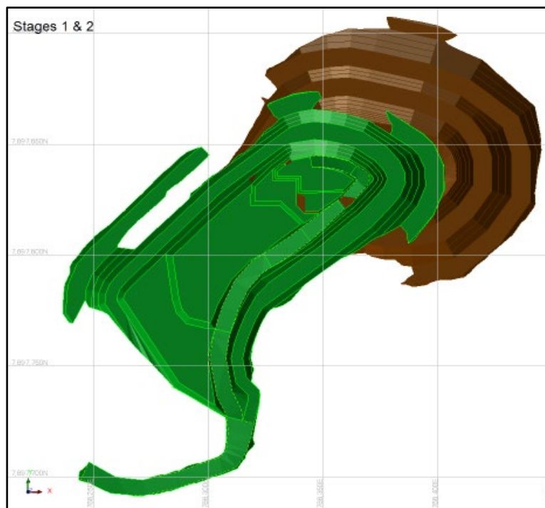
Figure 3 - Basic pit outlines: Green Stage 1 cut back which will produce around 18,000t of ore material; Brown Stage 2 cut back which will produce an additional 25,000t of ore material
