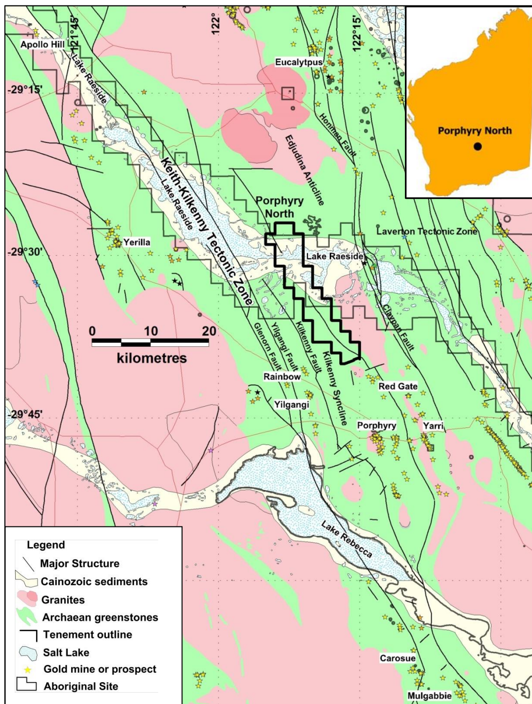
Figure 1: Porphyry North Project location within the Keith-Kilkenny Zone between the new Apollo Hill discovery and the Porphyry and Carosue Dam gold mines. Stars show gold mines and prospects.
