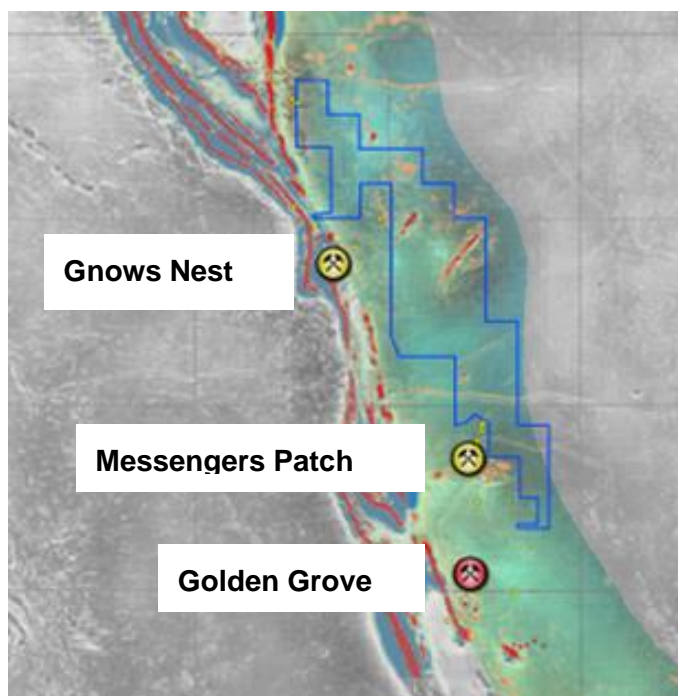
Messenger Project with magnetic imagery and nearby mines
