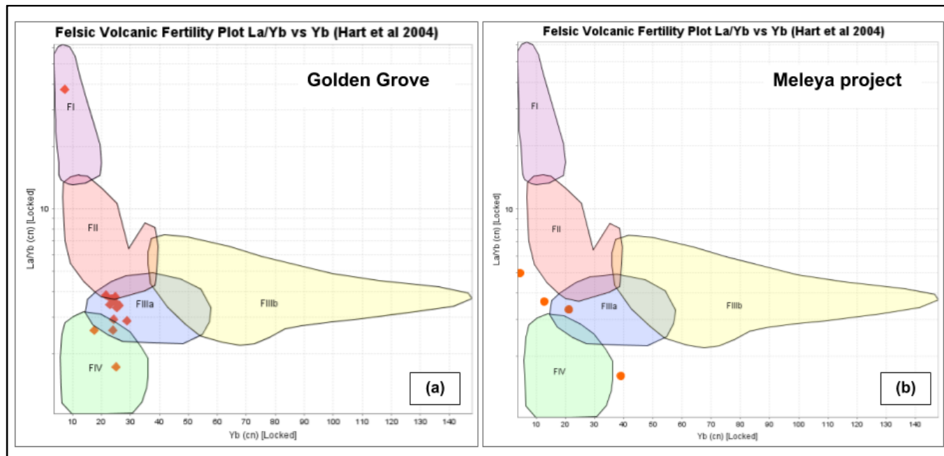
Plot of La/Yb vs Yb as proxy for fertility receptor for VMS (F1 Purple being non-fertile)
