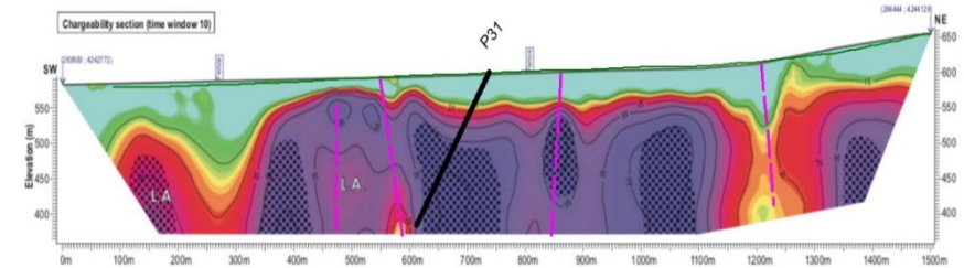
IP chargeability anomalies on survey line 16 showing location of proposed exploration drill hole P31
