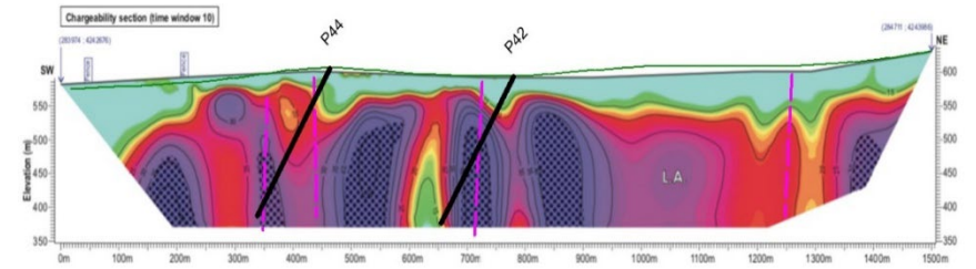
IP chargeability anomalies on survey line 18 showing location of proposed exploration drill holes P42 & P44
