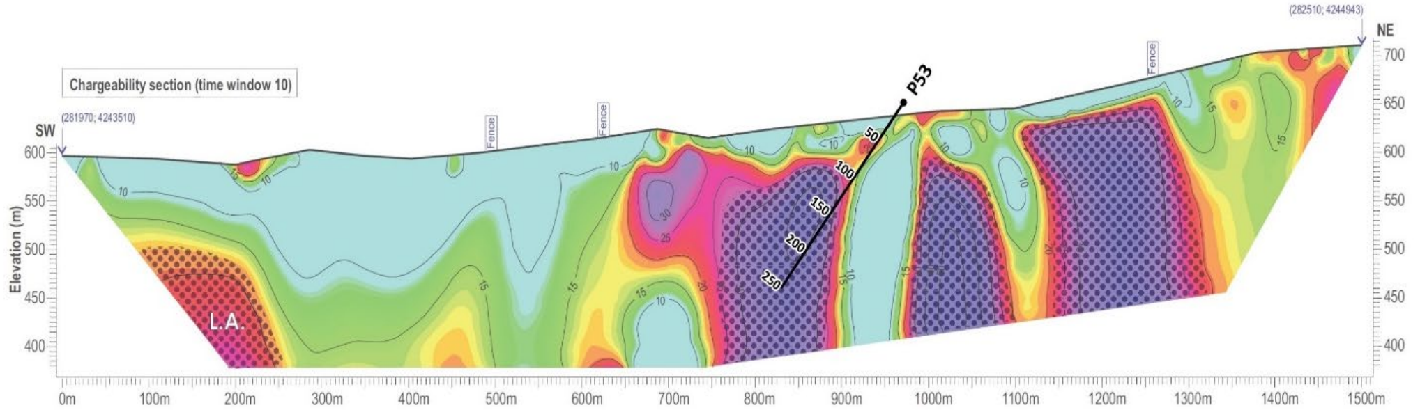
Cross-section of the location of Exploration drill hole P53 overlain on section of chargeability for IP line W4
