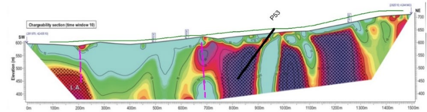
IP chargeability anomalies on survey line W4 showing location of proposed exploration drill hole P53
