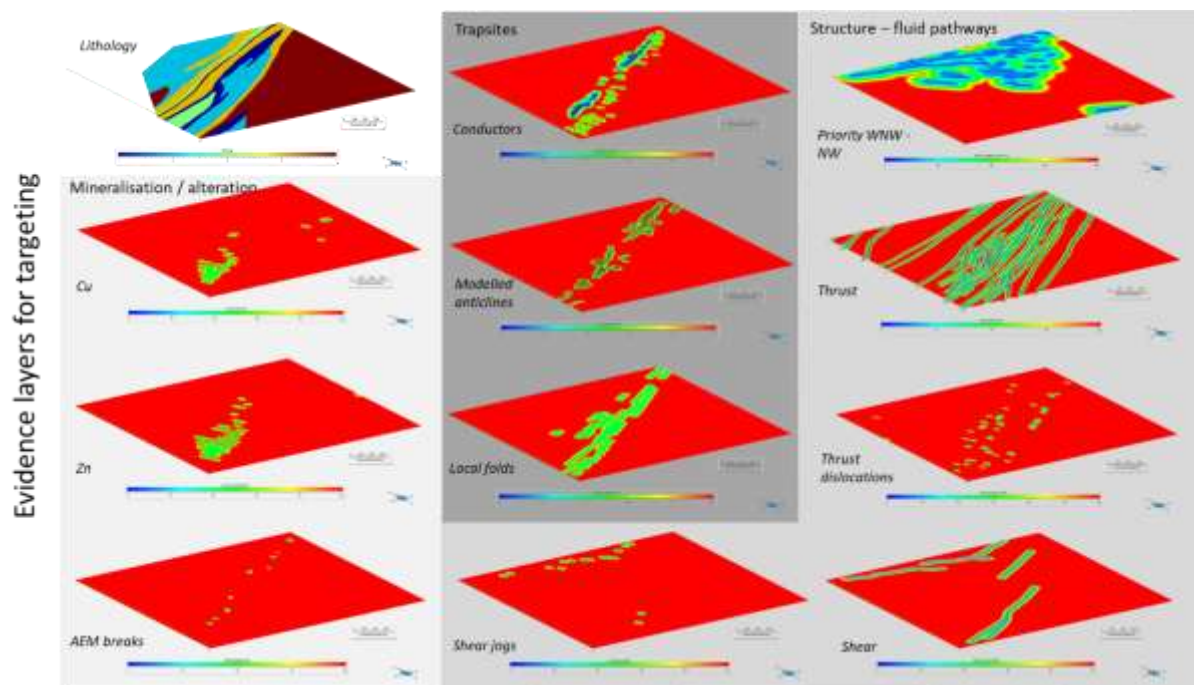
Figure 6. Examples of different evidence layers used for targeting. Layers are defined in terms of distance to- properties.
