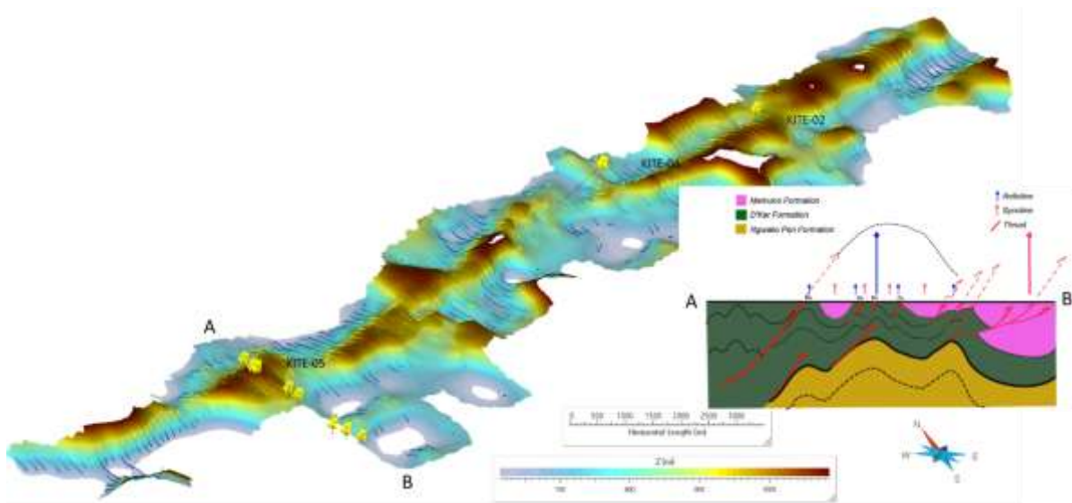
Figure 5. Section based 3D interpretation of AEM data highlighting anticline fold axis. Inset of geological interpretation based on drilling and AEM modelling.
