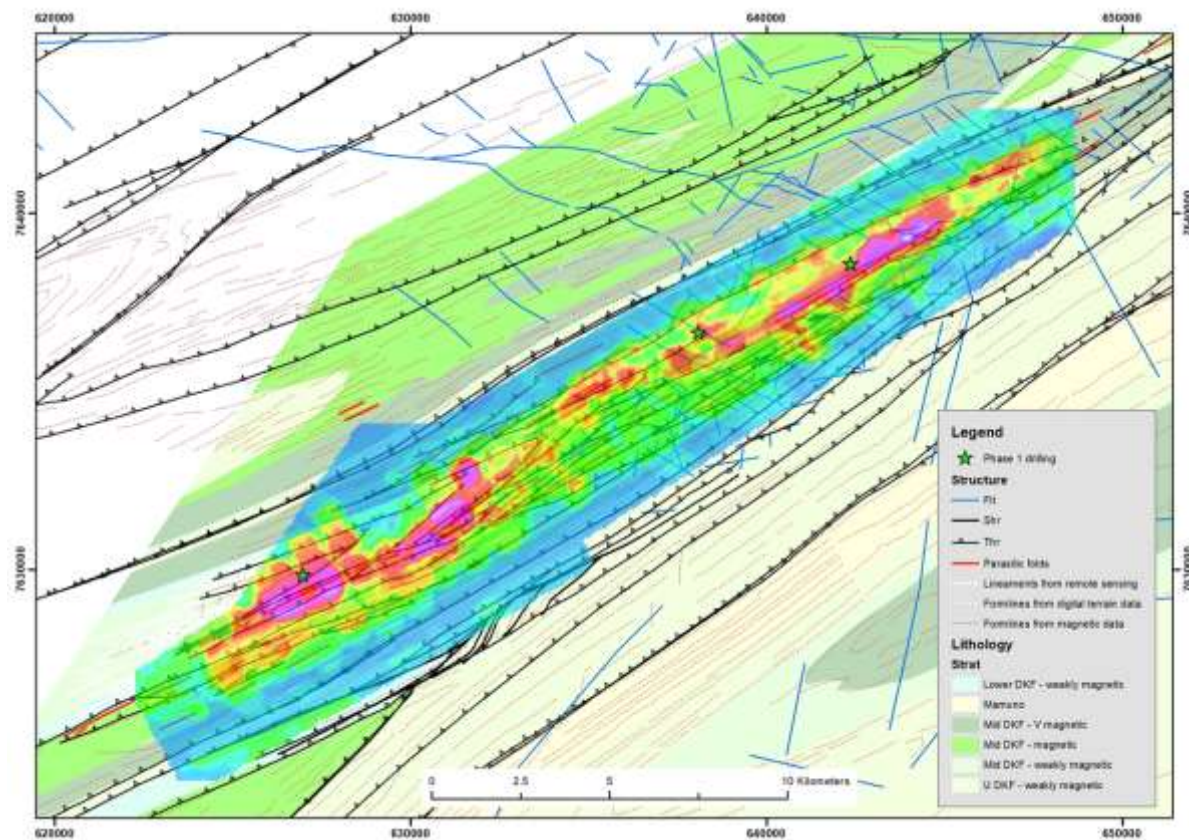
Figure 7. Prospectivity map (blue to magenta) on lithostructural interpretation.
