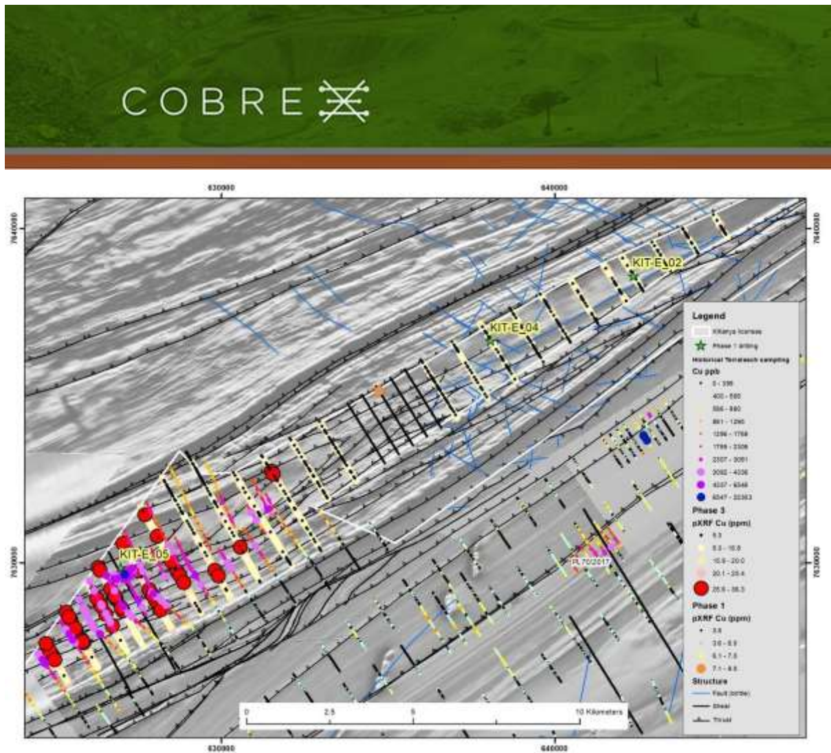
Figure 3. Soil sample results (Cu) on vertical derivative magnetic image.
