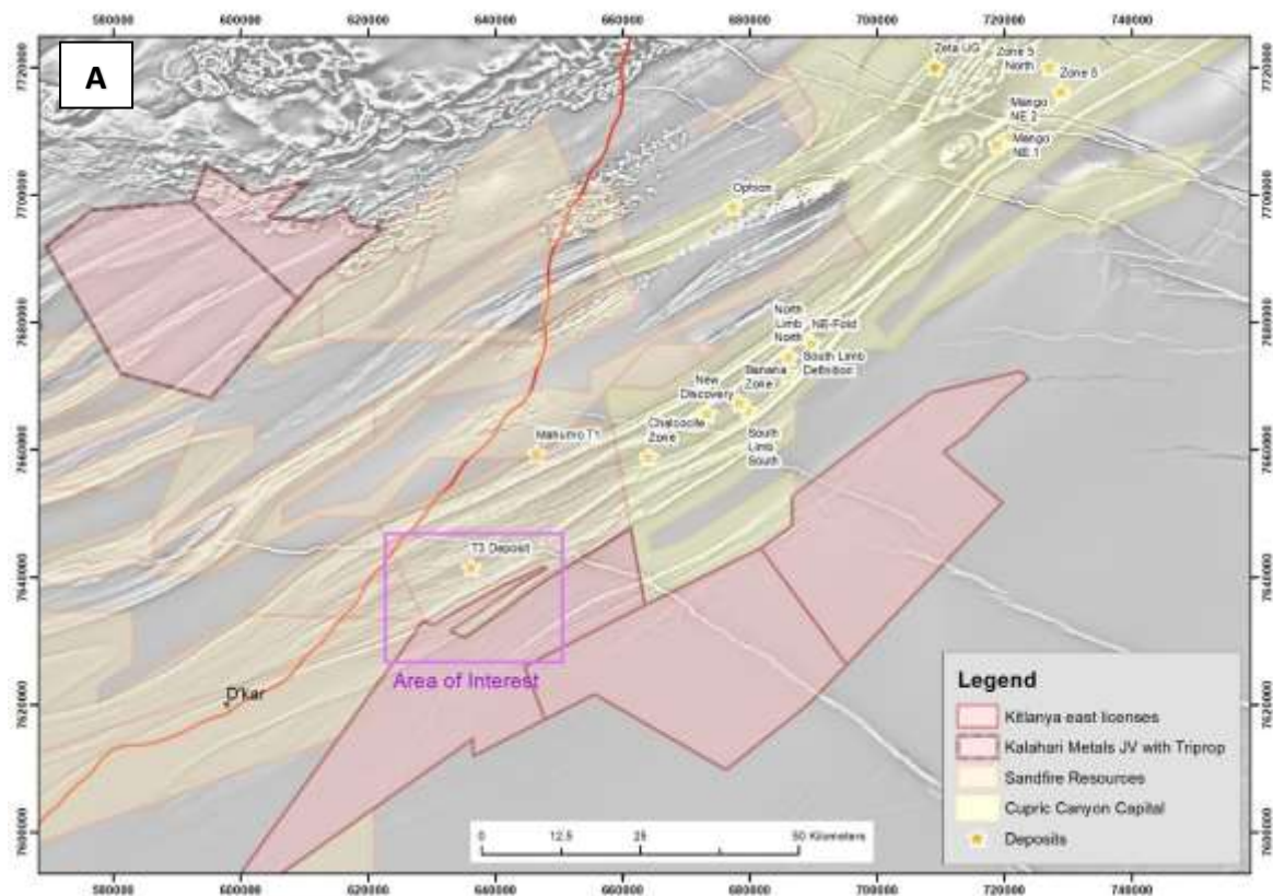
Figure 1. Locality map illustrating the position of the area of interest discussed in the current announcement relative to regional license holding in the Kalahari Copper Belt, NW Botswana. First vertical derivative greyscale total magnetic intensity background.
