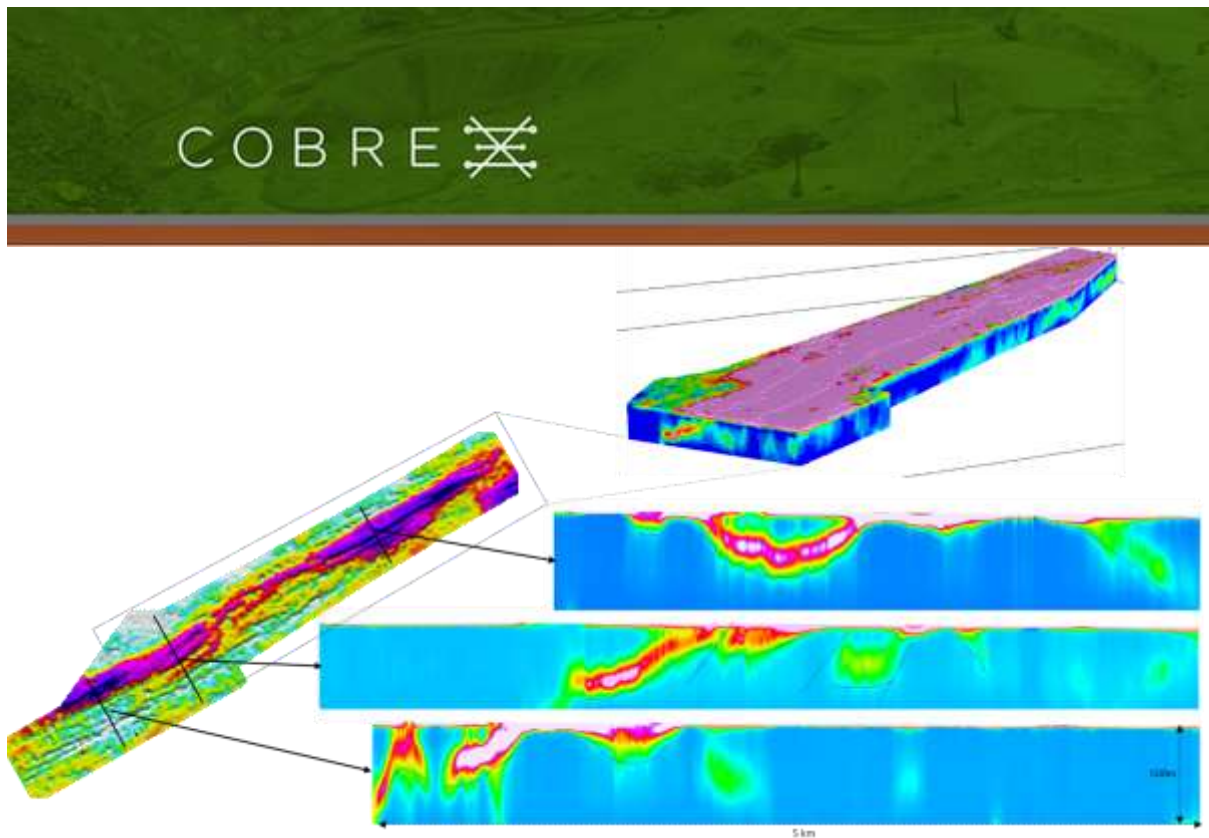
Figure 4. Conductivity sections and volume illustrating the significant structural detail apparent in the reprocessed AEM data.
