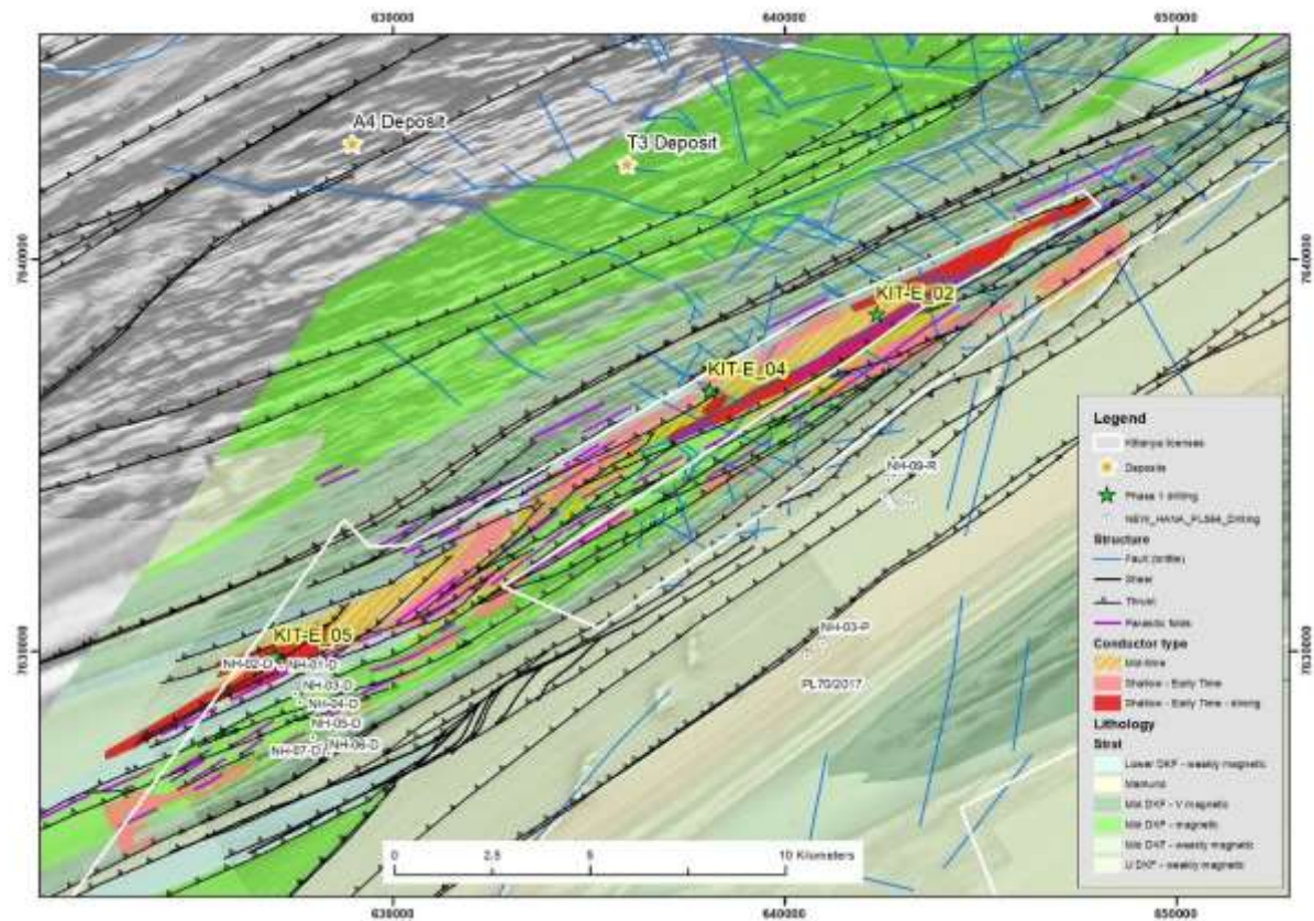
Figure 2. Locality map illustrating the position of recently completed stratigraphic holes along with historical drilling. Underlay of the lithostructural interpretation with AEM conductors highlighted on derivative image magnetic data.
