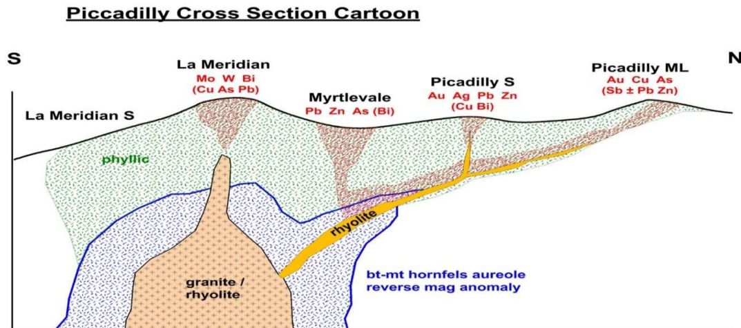
Figure 2: Schematic Model of Interpreted Intrusive Related mineral system at Piccadilly. Note idealised geological north south
