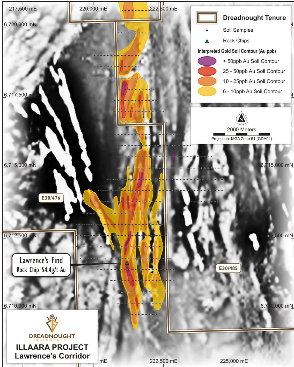
Figure 2: Plan view of the >10km long Lawrence’s Corridor highlighting gold-in-soil anomalies over a magnetics image and the location of Lawrence’s Find highlighted by the rock chip value.
