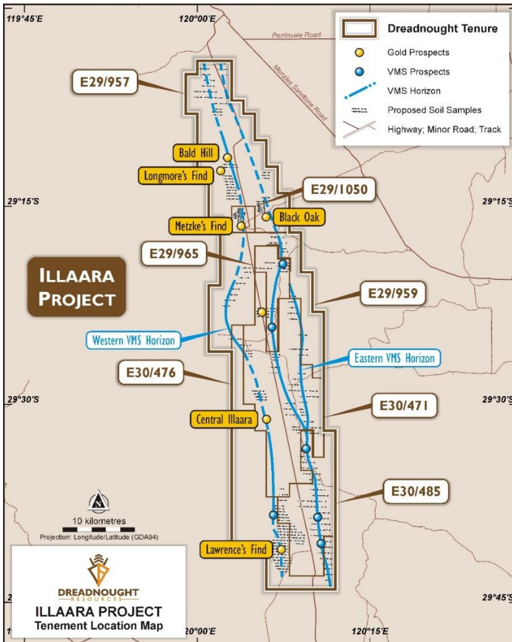
Figure 3: Plan view of Illaara showing the planned soil survey in relation to gold and VMS targets.
