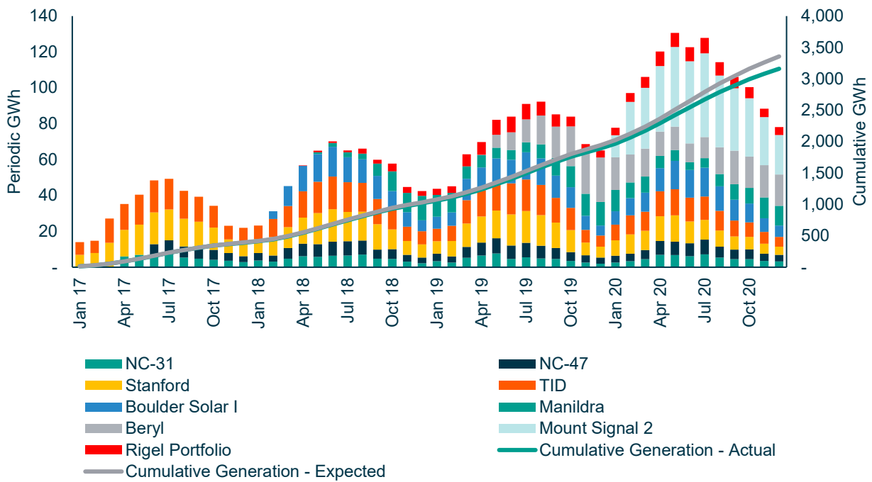
Figure 6: Operating Portfolio monthly generation 16
