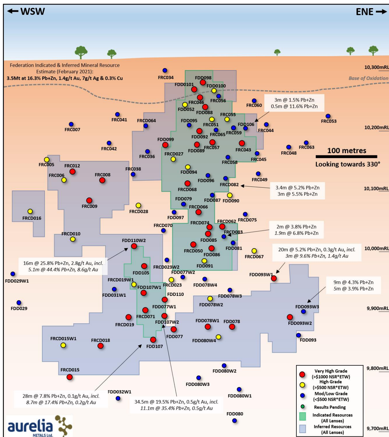
Figure 1. Schematic long section showing the Federation deposit with an outline of the Indicated and Inferred Resource areas and selected intercepts.
