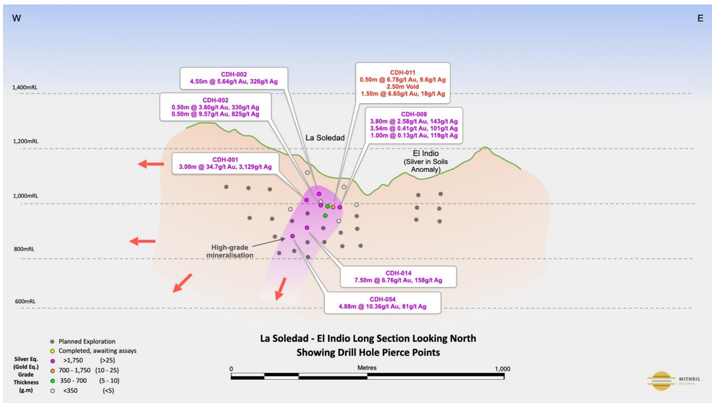
Figure 8: Long section La Soledad to El Indio showing drill hole pierce points and grade-thickness Silver Eq 1 x metres (Gold Eq.1 x metres), which has increased with depth. Long section location shown above in Figure 2 (red).
