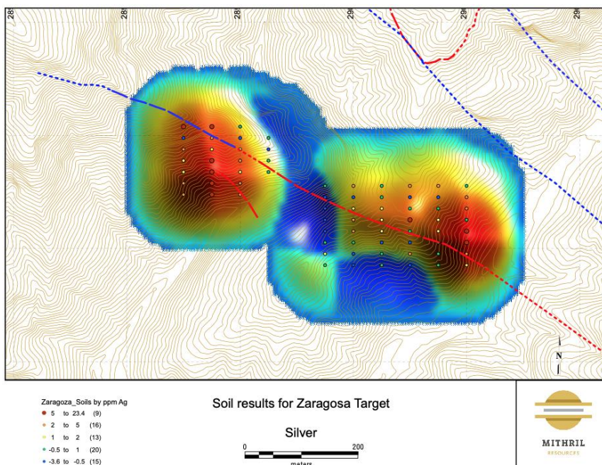
Figure 15 Heat map (silver grades ppm) for the Zaragoza target soil sampling located just to the SE of the El Refugio target.
