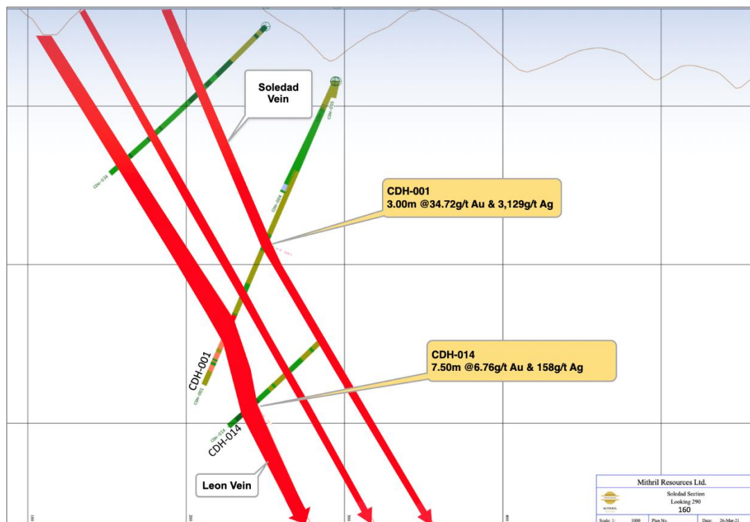
Figure 11 Cross Section 160 at La Soledad target showing hole CDH-001 and hole CDH-014
