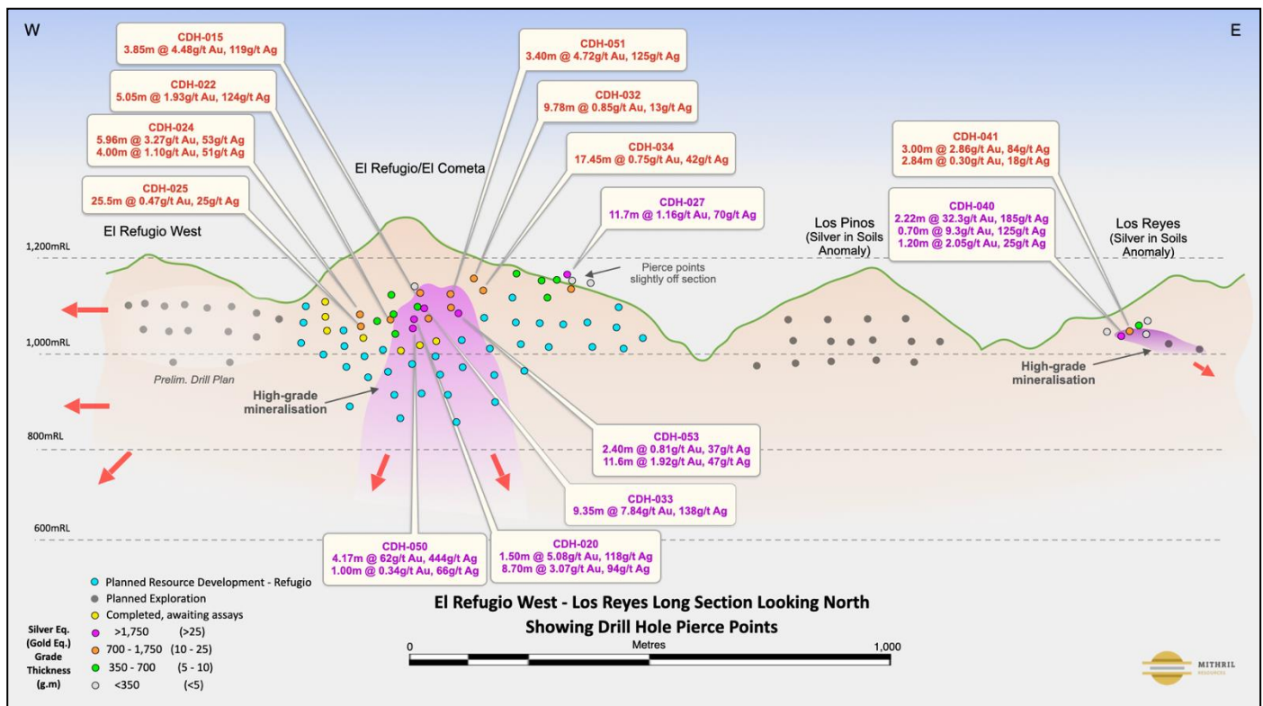
Figure 1: Long section El Refugio West to Los Reyes showing drill hole pierce points and grade-thickness Silver Eq 1 x metres (Gold Eq. 1 x metres), which has increased with depth. Long section location shown below in Figure 2 (orange).
