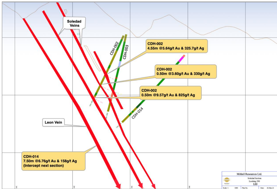
Figure 10 Cross Section 120 at La Soledad target showing hole CDH-002 and hole CDH-014 (intercept next section)
