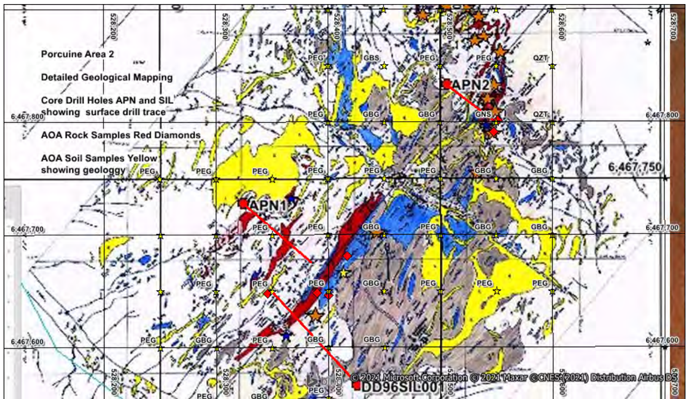
Figure 5: EL 8747 Stirling Vale - Porcuine Prospect Area 2 showing the historical drill holes and drill hole traces in red
