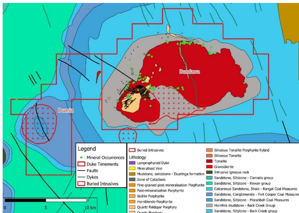
Figure 4. Local scale geology of the Bundarra tenement.
