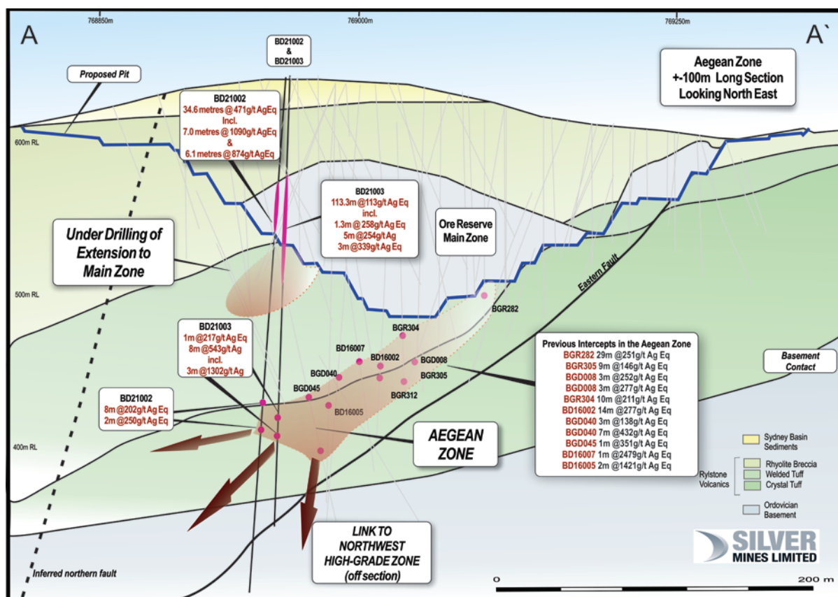
Figure 3: Section A-A' through Main Zone Ore Reserve and Aegean Zone showing new intercepts and previous intercepts.
